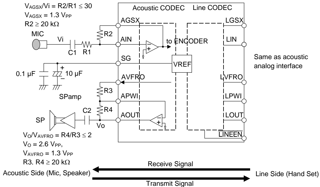
Figure 1 Analog Interface
