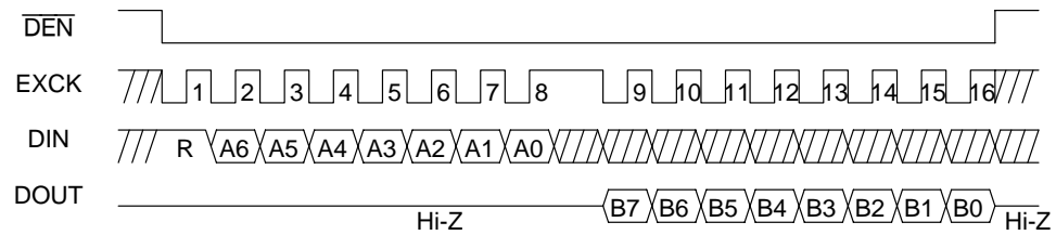
(c) Data Read Timing 1 (8-bit MCU)
