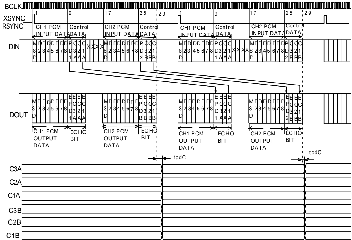
Figure 3 CONTROL BIT TIMING and ECHO BACK TIMING
