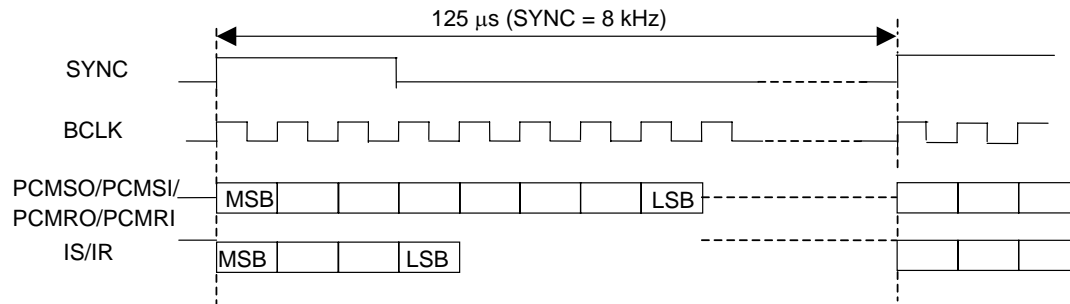
Figure 1 PCM and ADPCM Interface Basic Timing
