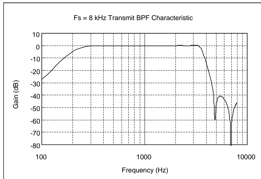
Figure 9 Transmit Bandpass Filter Characteristic (Fs = 8 kHz, CR3-B1, B0 = (0, 0))
