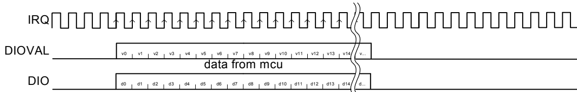
Figure 8. DIO Transmit Sequence
