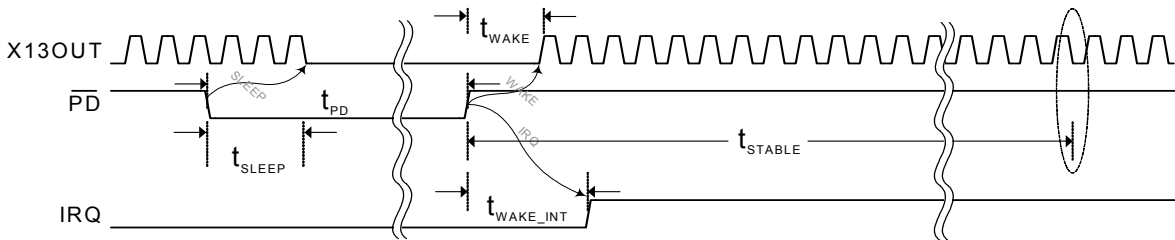
Figure 14. Sleep/Wake Timing
