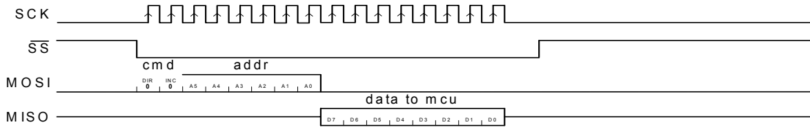
Figure 3. SPI Single Read Sequence
