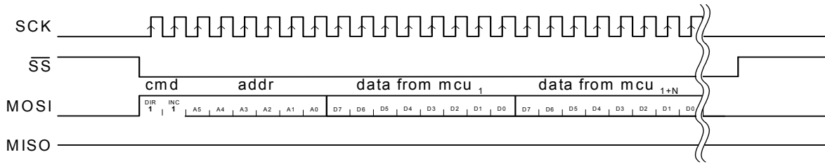
Figure 6. SPI Burst Write Sequence
