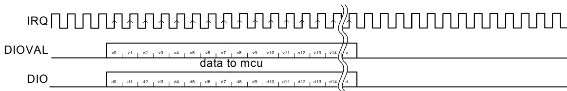
Figure 7. DIO Receive Sequence
