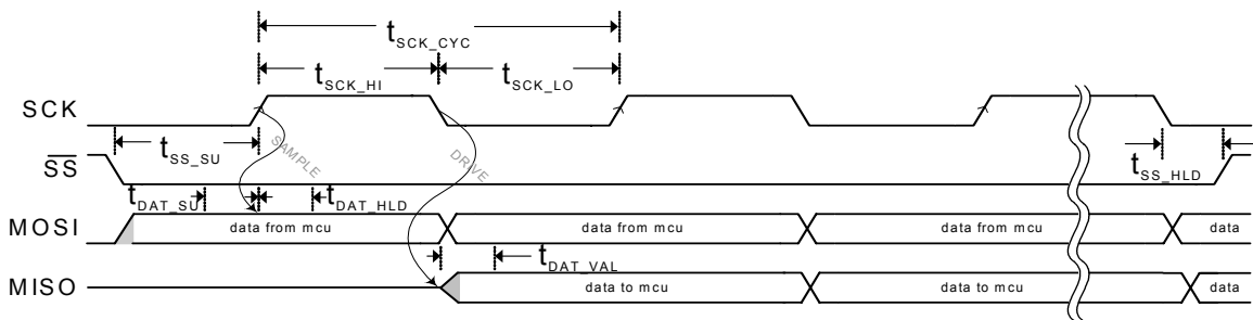
Figure 9. SPI Timing Diagram
