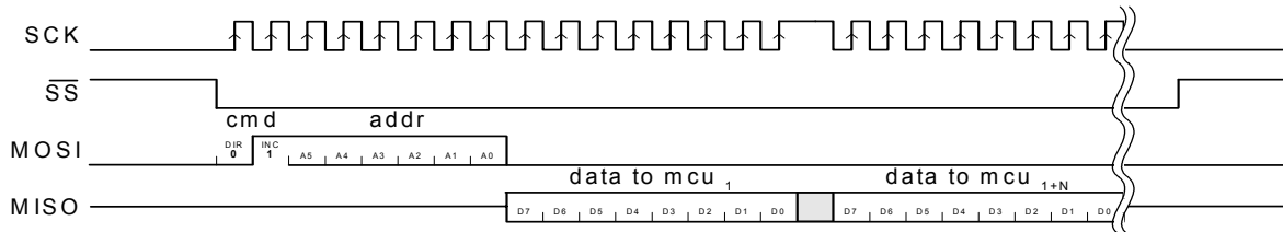
Figure 4. SPI Burst Read Sequence
