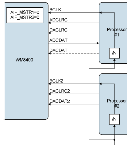
Figure 63 Interface 1 = Slave, Interface 2 = Slave
