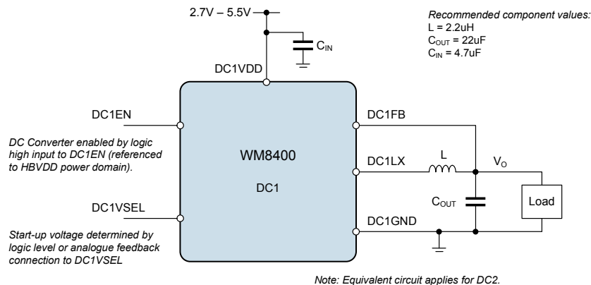
Figure 106 DC-DC Converter External Components
