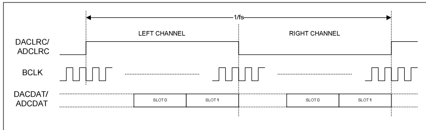
Figure 76 TDM in Right-Justified Mode
