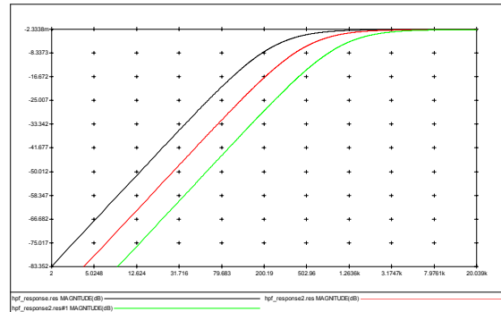
Figure 90 ADC Digital High Pass Filter Ripple (48kHz, Voice Mode, ADC_HPF_CUT=01, 10 and 11)
