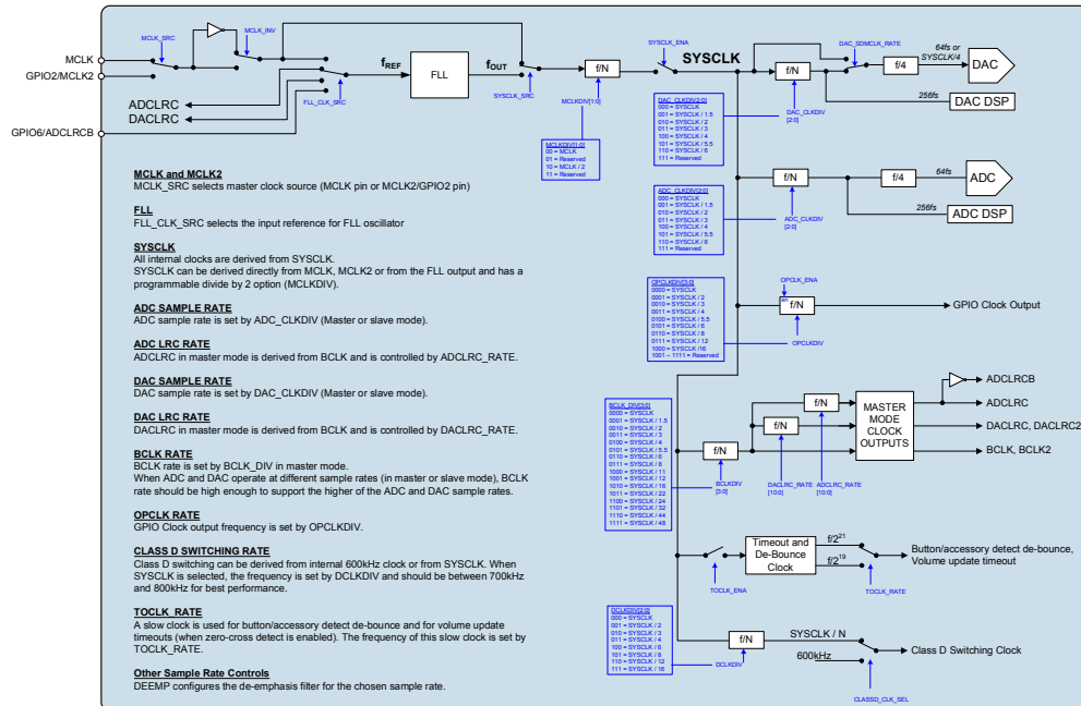
Figure 17 CODEC Clocking Scheme
