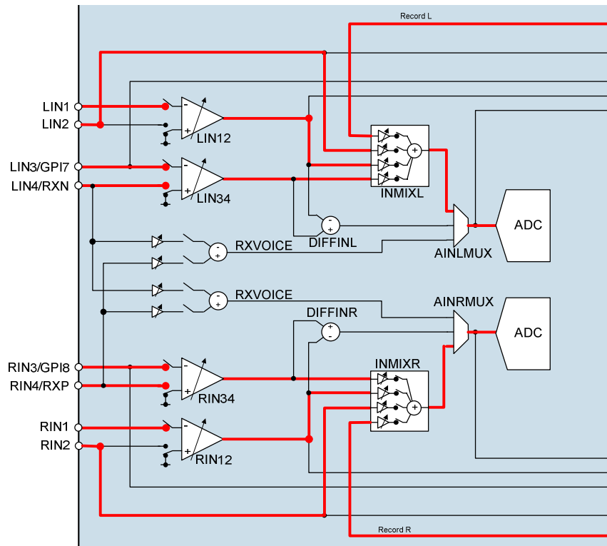
Figure 28 Mixer Mode Signal Paths
