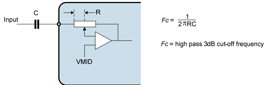
Figure 101 Audio Input Path DC Blocking
