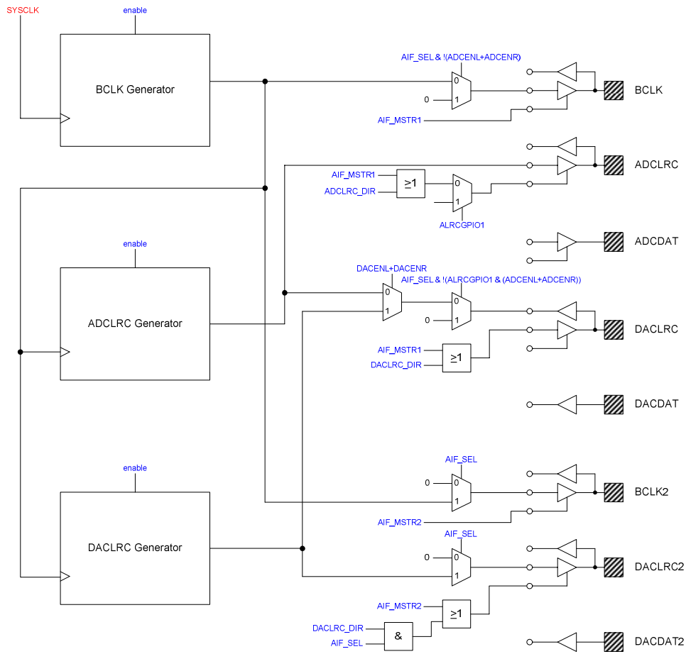
Figure 65 Audio Interface Output Control
