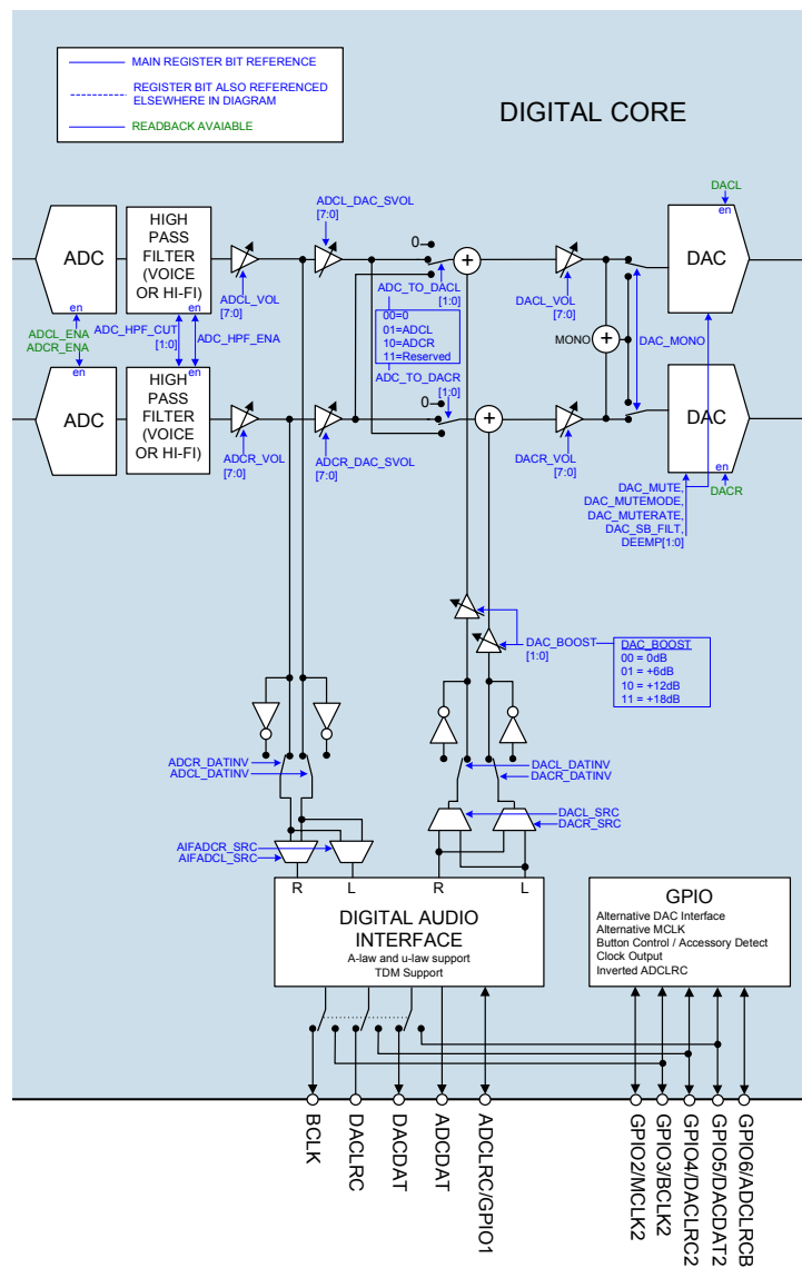
Figure 31 Digital Mixing Paths
