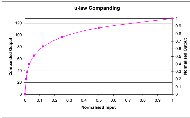
Figure 82 \mu -Law Companding
