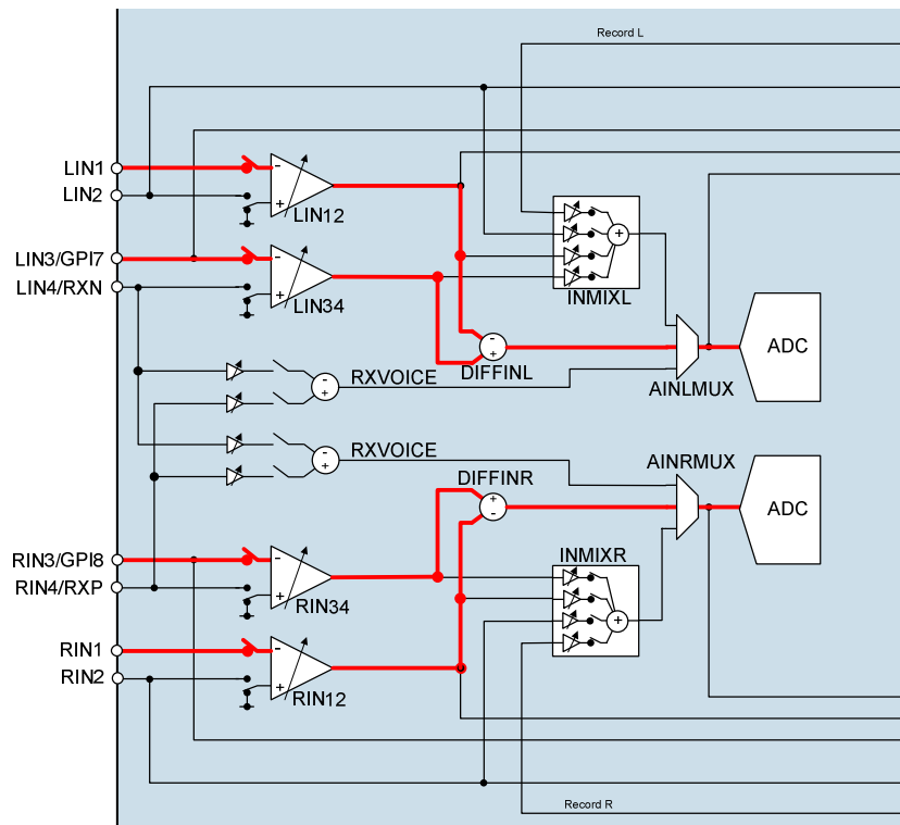
Figure 30 Differential Mode Signal Paths
