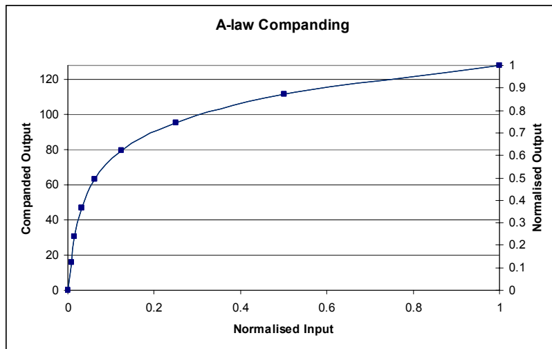
Figure 83 A-Law Companding
