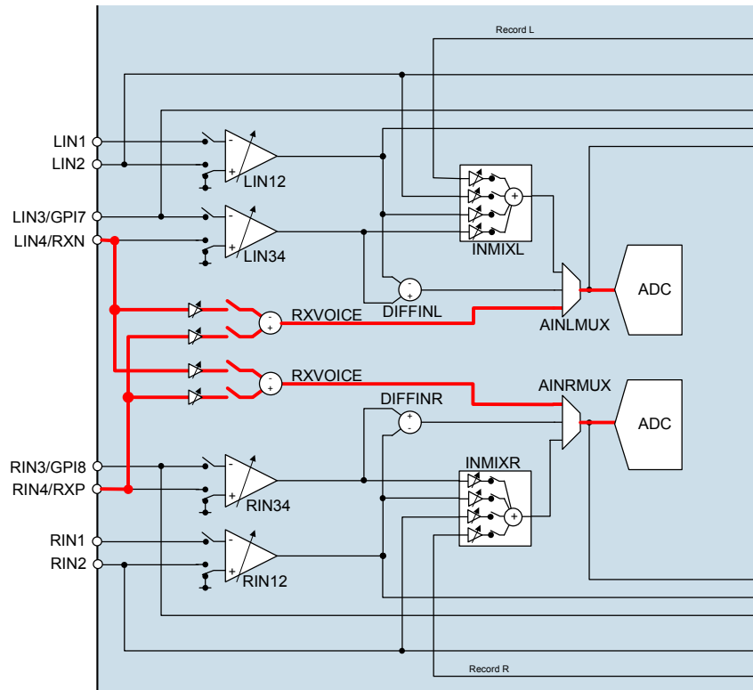
Figure 29 RxVoice Mode Signal Paths
