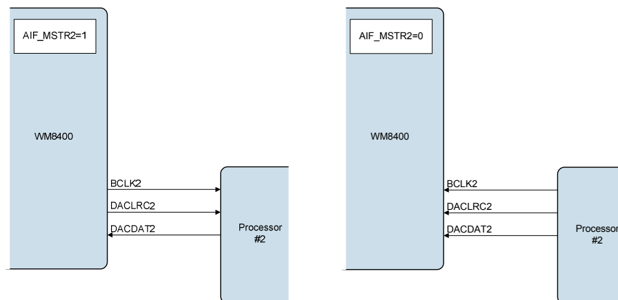
Figure 58 Interface 2 = Master
