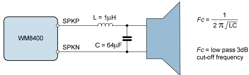
Figure 104 Class D Output Filter Components
