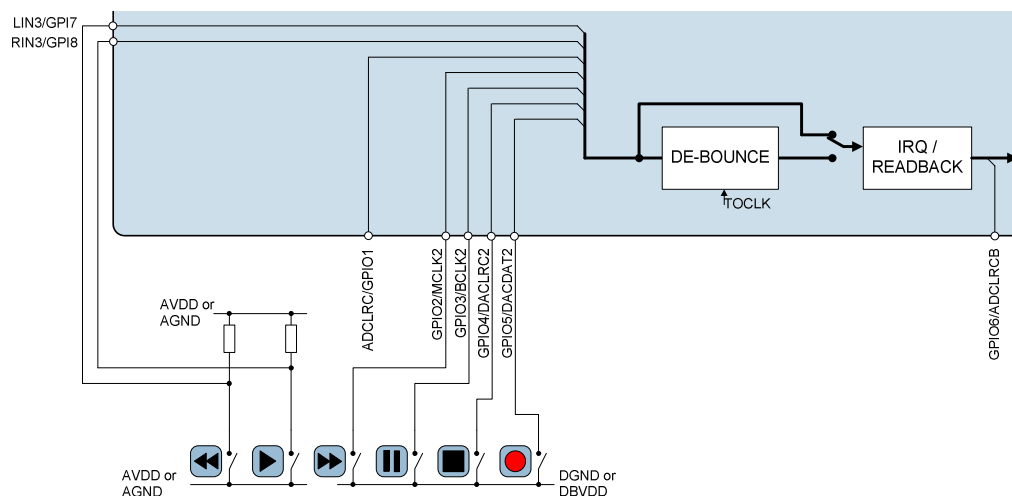
Figure 46 Example of Button Control Using GPIO Pins
