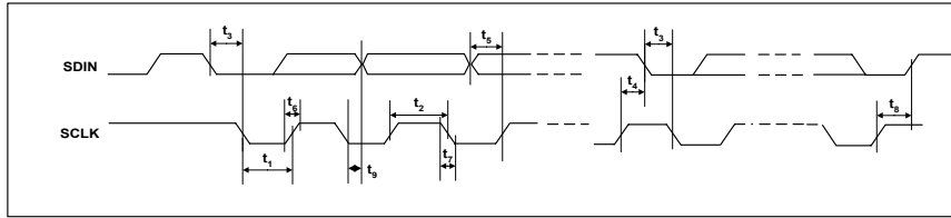
Figure 6 Control Interface Timing – 2-Wire Serial Control Mode
