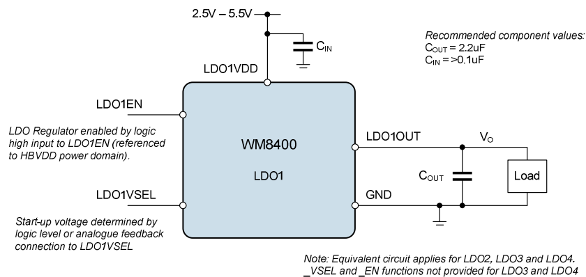
Figure 107 LDO Regulator External Components
