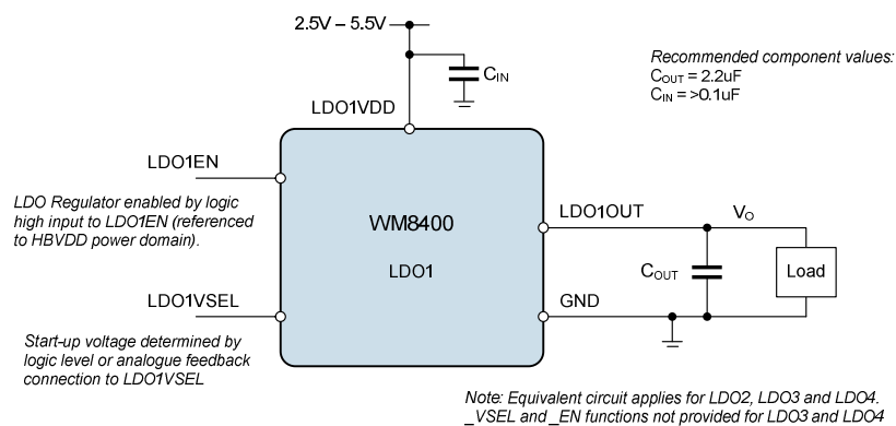
Figure 86 LDO Regulator Connections
