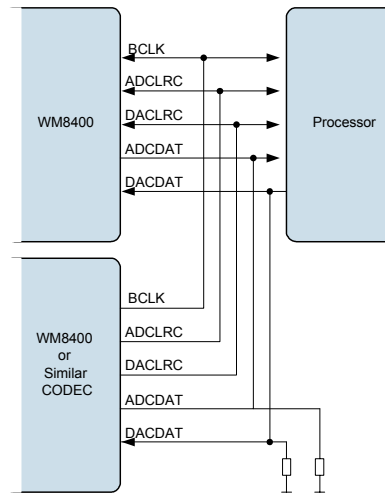
Figure 67 TDM with Other CODEC as Master
