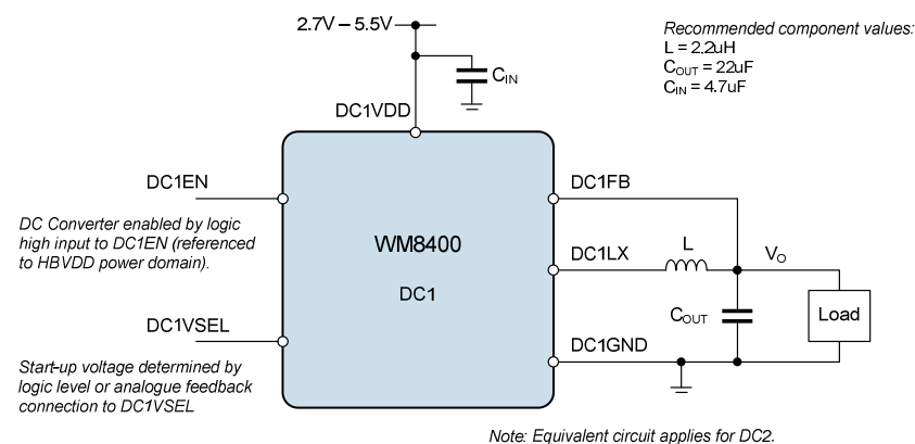
Figure 85 DC-DC Converter Connections
