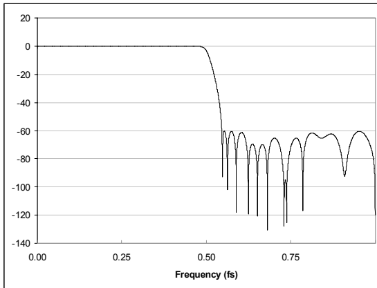
Figure 87 ADC Digital Filter Frequency Response
