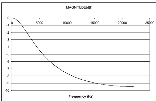
Figure 97 De-Emphasis Digital Filter Response (44.1kHz)
