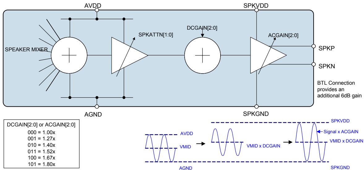
Figure 34 Speaker Boost Operation
