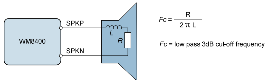
Figure 105 Speaker Equivalent Circuit for Filterless Operation
