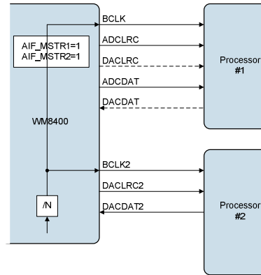
Figure 60 Interface 1 = Master, Interface 2 = Master
