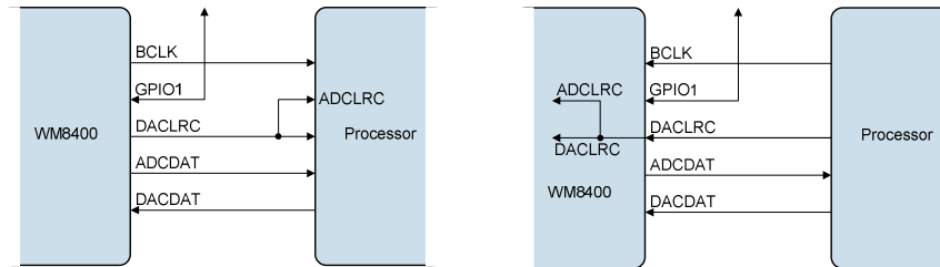
Figure 56 Master Mode with ADCLRC as GPIO Figure 57 Slave Mode with ADCLRC as GPIO
