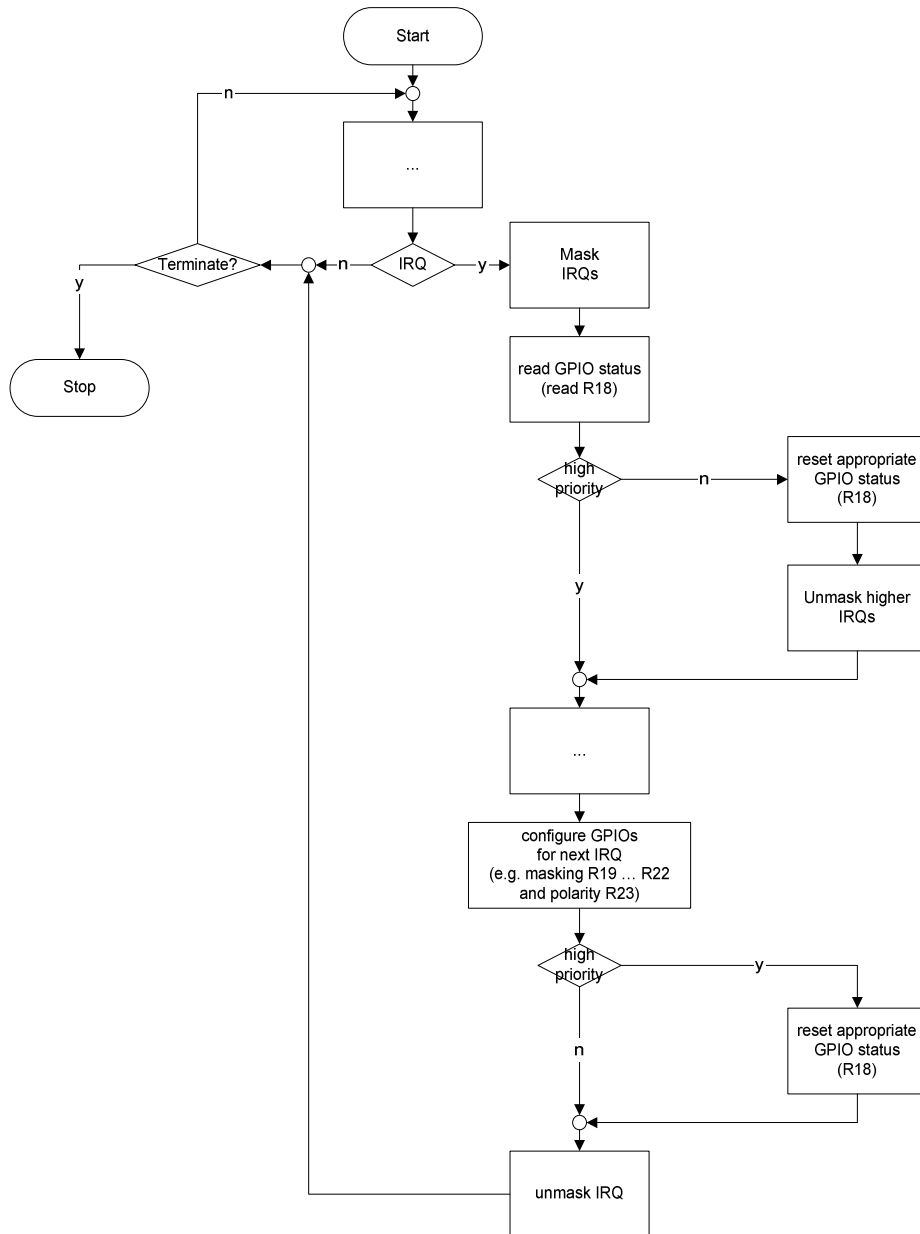
Figure 53 GPIO IRQ Handling
