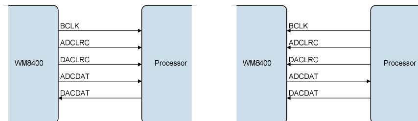
Figure 54 Master Mode
