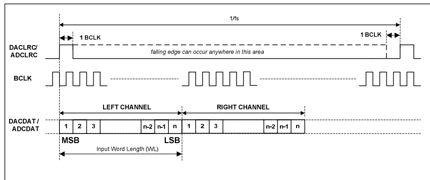
Figure 75 DSP Mode Audio Interface (mode B, AIF_LRCLK_INV=1, Slave)
