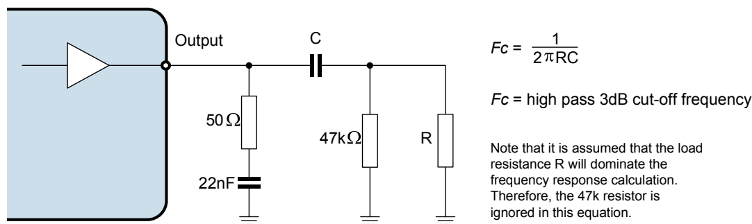
Figure 102 Audio Output Path Components
