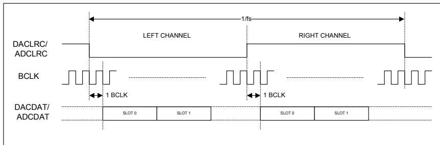
Figure 78 TDM in I²S Mode
