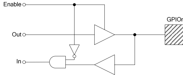
Figure 48 GPIO Pad
