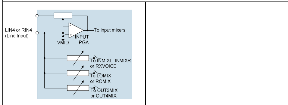
Figure 27 LIN4 or RIN4 as Line Inputs
