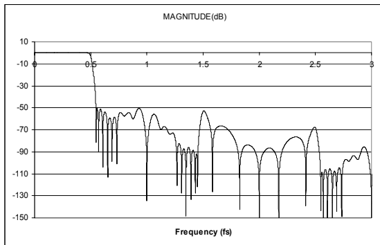
Figure 91 DAC Digital Filter Frequency Response (Normal Mode)
