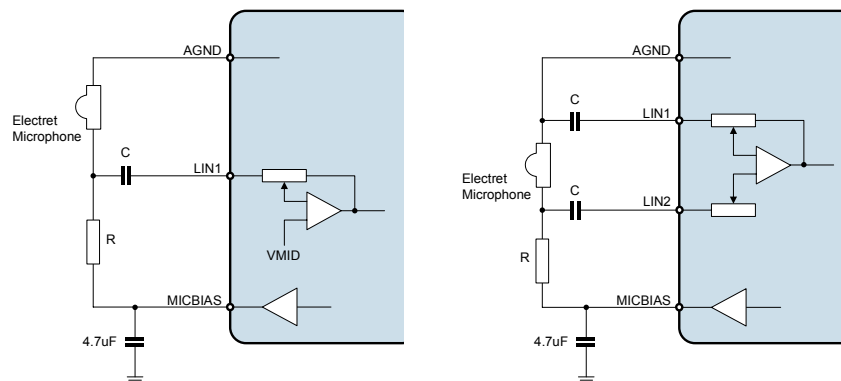
Figure 103 Single-Ended and Pseudo-Differential Microphone Connections
