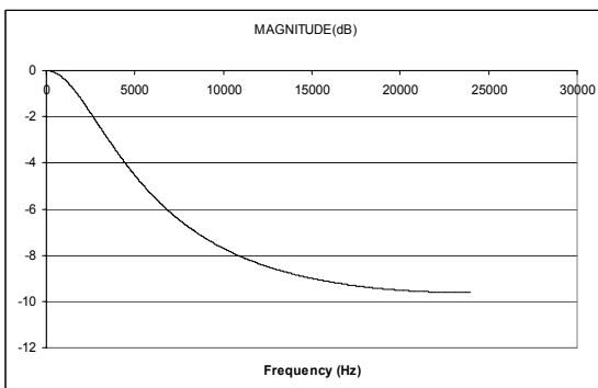
Figure 99 De-Emphasis Digital Filter Response (48kHz)
