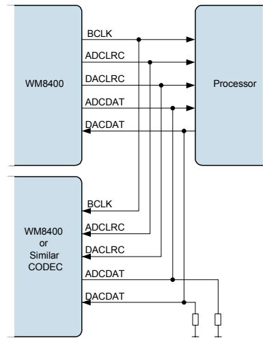
Figure 66 TDM with WM8400 as Master
