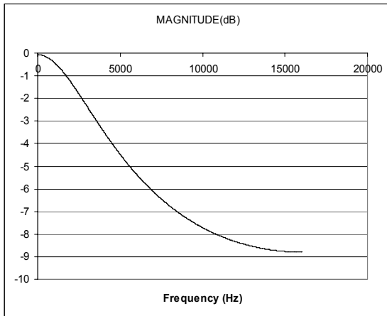
Figure 95 De-Emphasis Digital Filter Response (32kHz)
