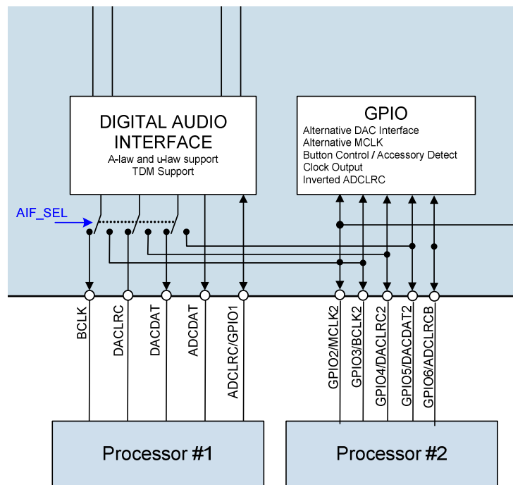
Figure 45 Alternative DAC Interface
