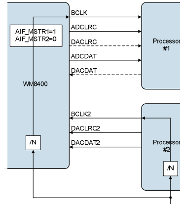
Figure 61 Interface 1 = Master, Interface 2 = Slave
