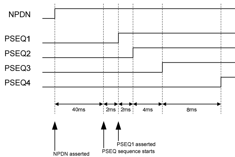
Figure 84 Power Sequencing Timing
