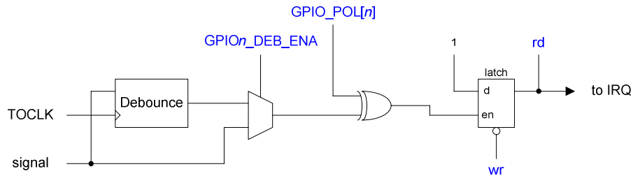
Figure 49 GPIO Function
