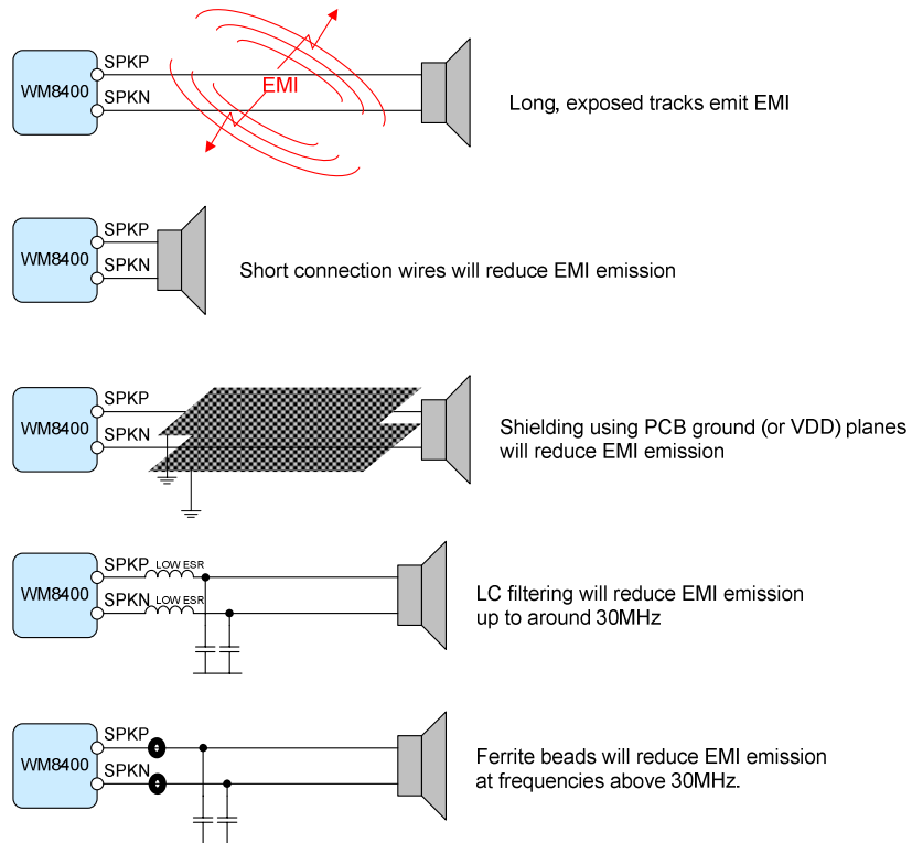
Figure 108 EMI Reduction Techniques
