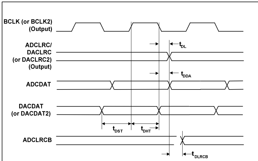
Figure 3 Digital Audio Data Timing - Master Mode (see Control Interface)
