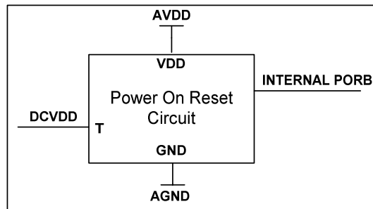
Figure 9 Internal Power on Reset Circuit Schematic
