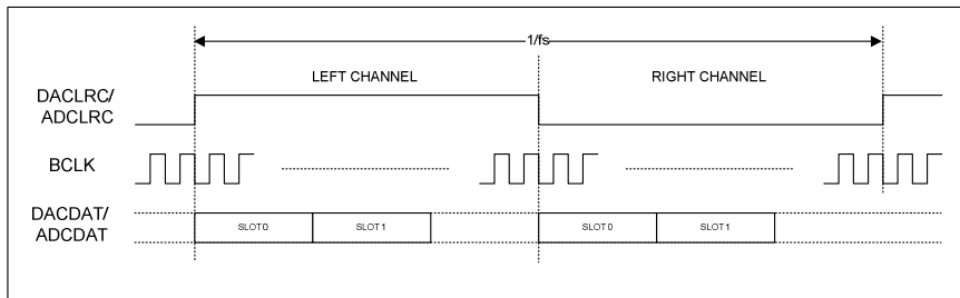
Figure 77 TDM in Left-Justified Mode
