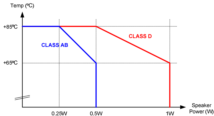
Figure 1 Speaker Power De-Rating Curve
