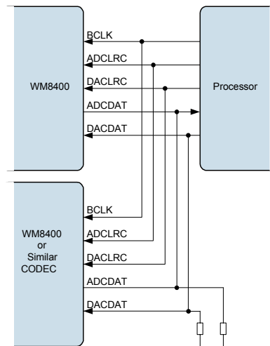
Figure 68 TDM with Processor as Master
