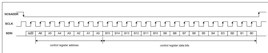
Figure 16 3-Wire Serial Control Interface
