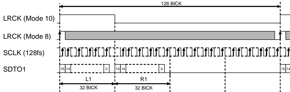
Figure 5. Mode 8, 10 Timing (TDM128A mode, MSB justified)
