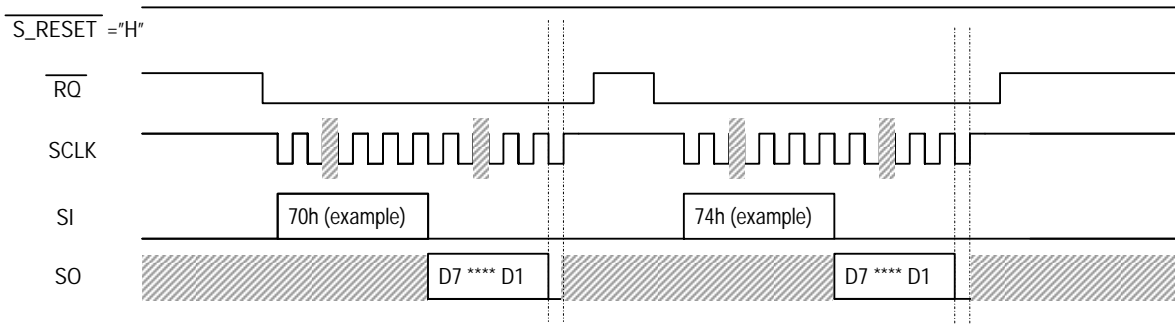
Fig.8-30 Control register read (during RUN phase)
