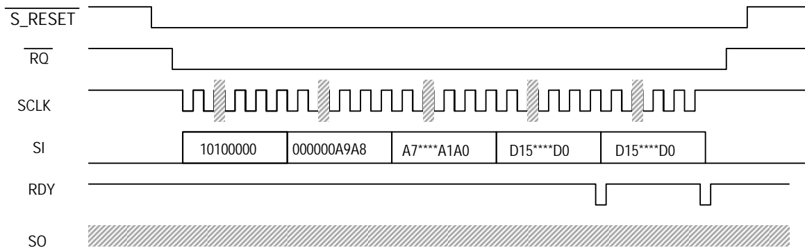
Fig.8-18 Input of continuous address data into CRAM
