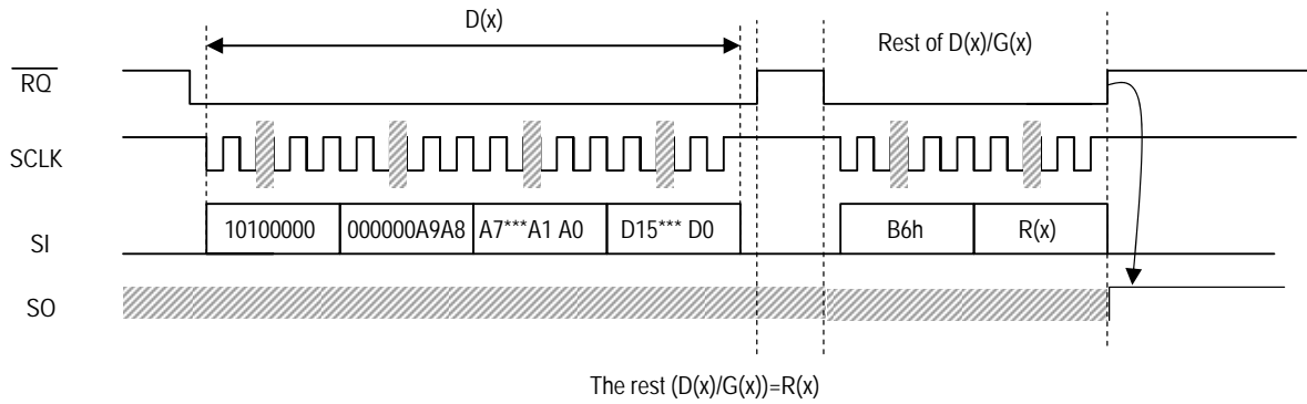
Fig.8-33 The rest of D(x)/G(x)=R(x) CRC Check example.
