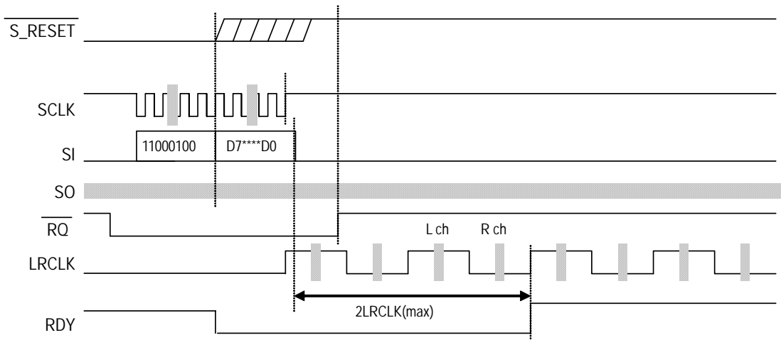
Fig.8-22 Timing for external conditional jump write operation (during reset phase)
