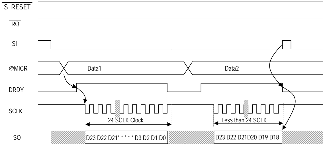
Fig.8-31 SO read (during RUN phase)
