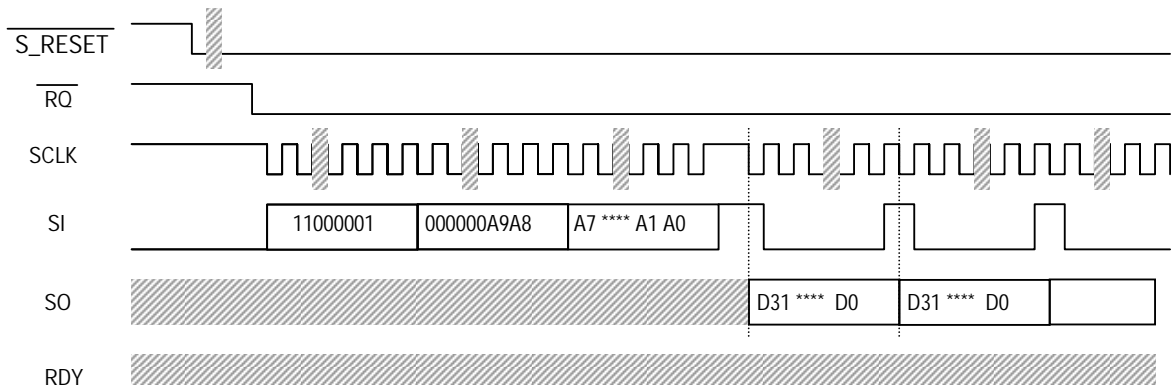
Fig.8-24 Reading of PRAM data
