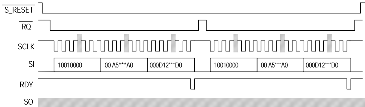
Fig.8-21 Input of discontinuous address data into OFRAM
