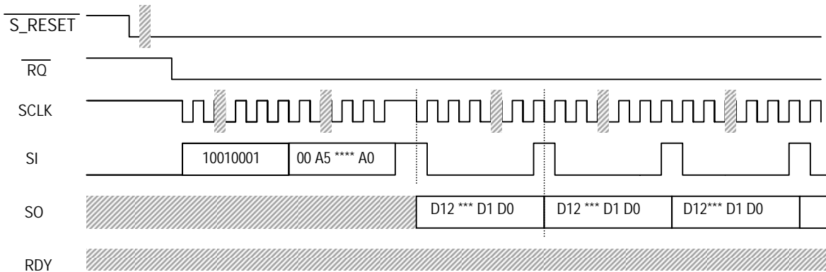
Fig.8-26 Reading of OFRAM data
