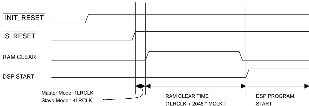
Fig.8-7 RAM CLEAR SEQUENCE
