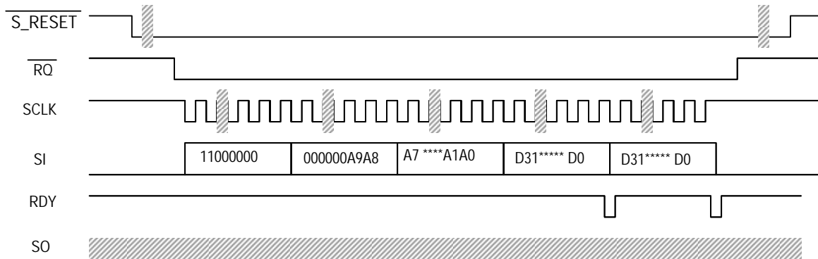
Fig.8-16 Input of continuous address data into PRAM
