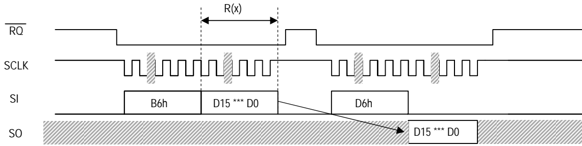
Fig.8-32 Example: Control register writing, reading
