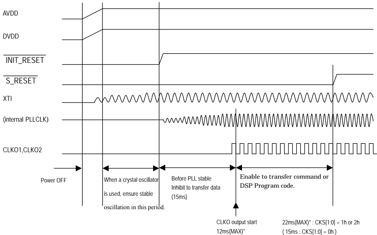
Fig.8-6 Power supply startup sequence
