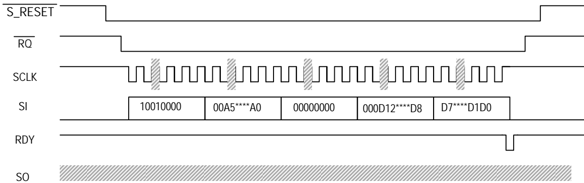
Fig.8-20 Input of data into OFRAM
