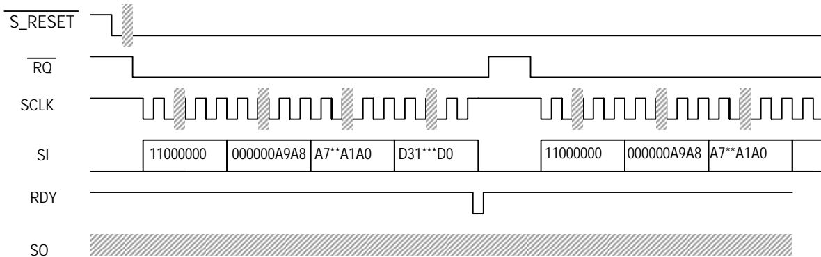
Fig.8-17 Input of discontinuous address data into PRAM
