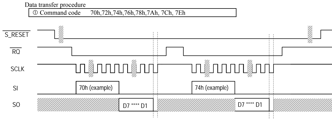
Fig.8-23 Reading of Control Register data
