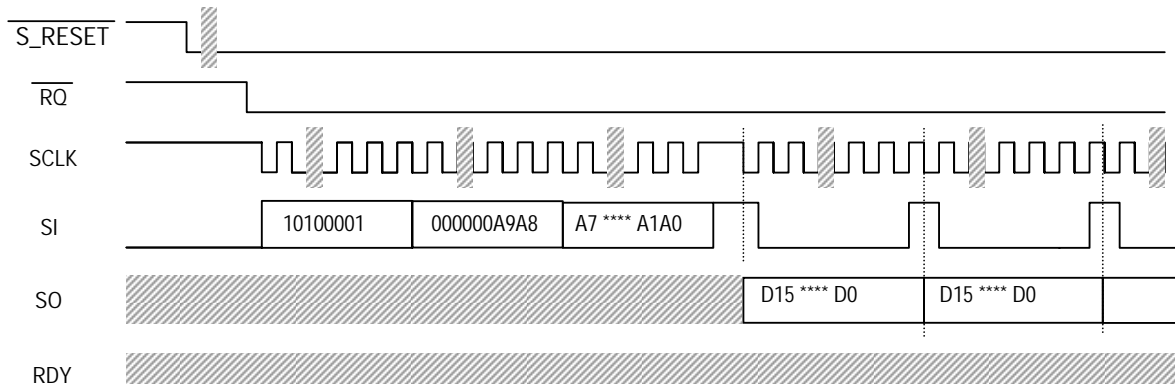
Fig.8-25 Reading of CRAM data
