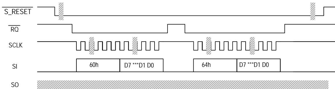
Fig .8-15 Control Registers write operation
