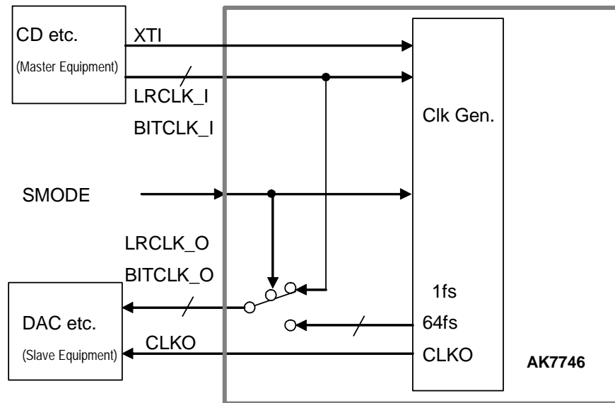
Fig. 8-9 Slave mode example
