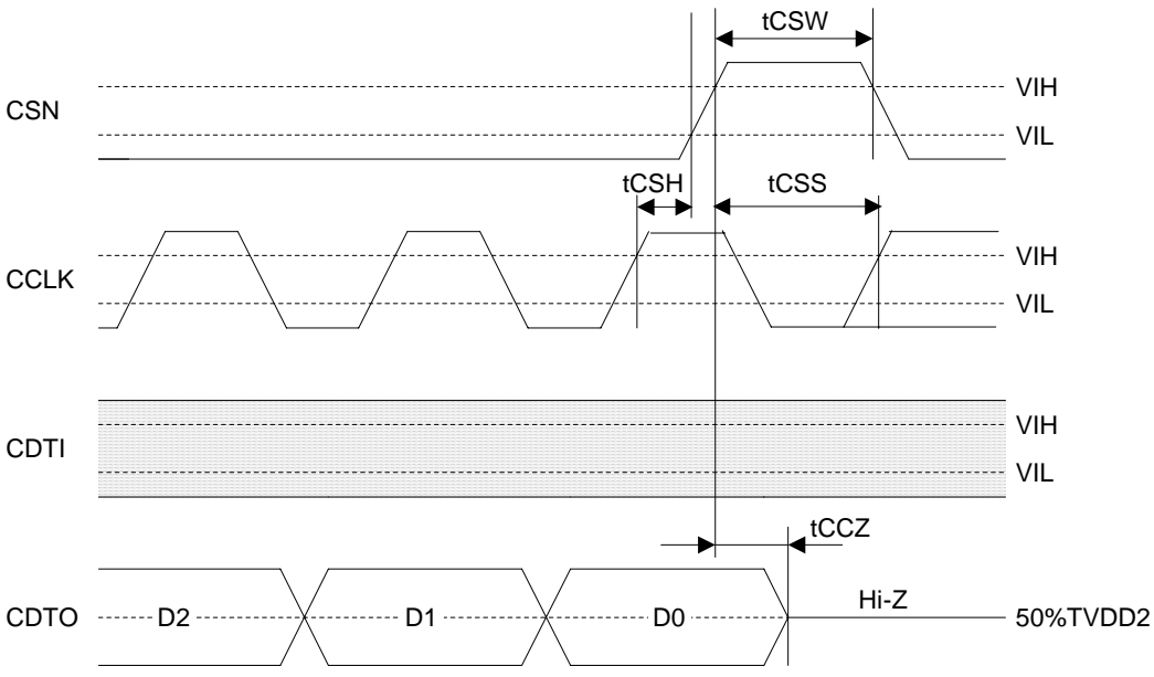
Figure 14. Read Data Output Timing2(4-wire Serial mode)
