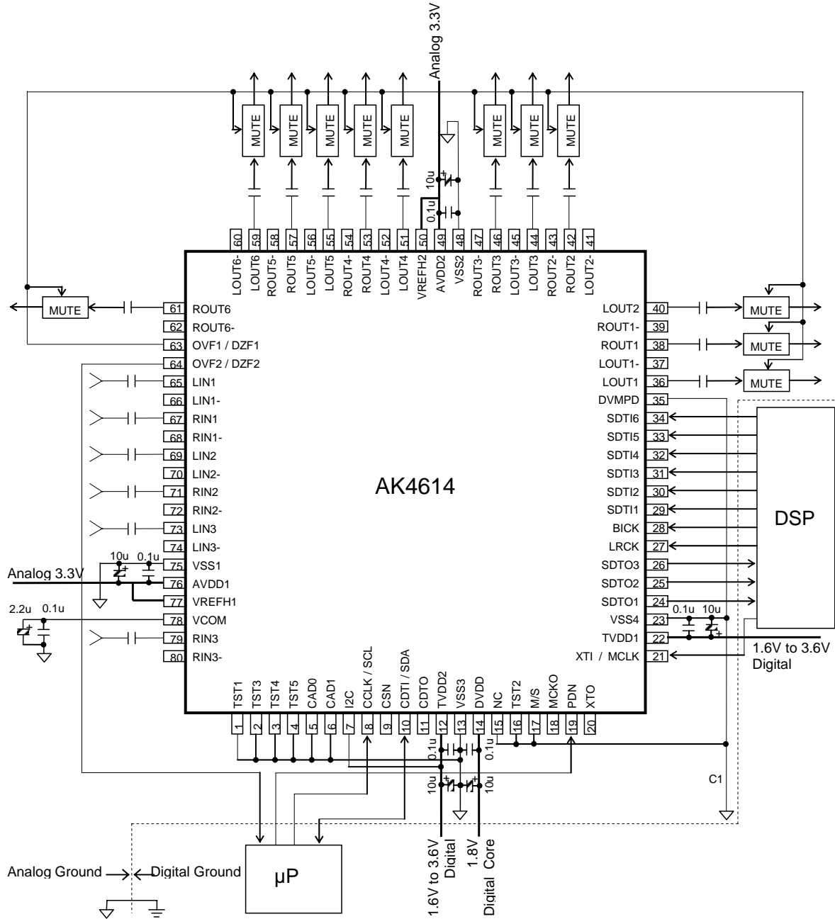
Figure 60. Typical Connection Diagram2
