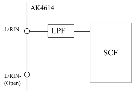
Figure 20. Single-end Input (DIE1-3 bit = “0”)
