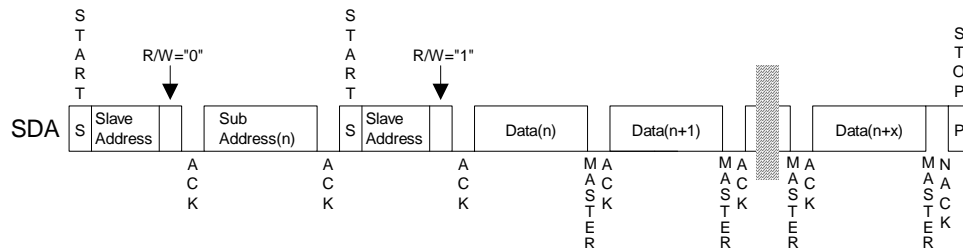
Figure 55. RANDOM ADDRESS READ
