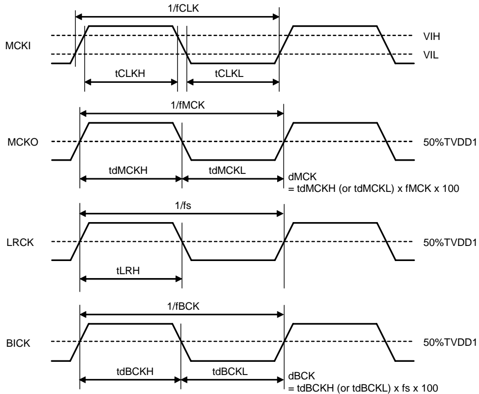
Figure 6. Clock Timing (Except TDM1/0 bit = "00" & Master mode)
