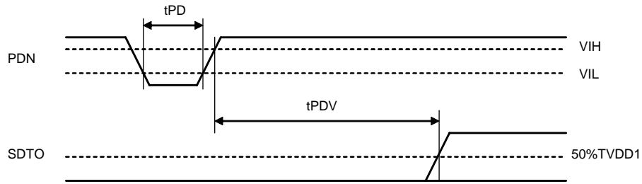
Figure 16. Power-down & Reset Timing
