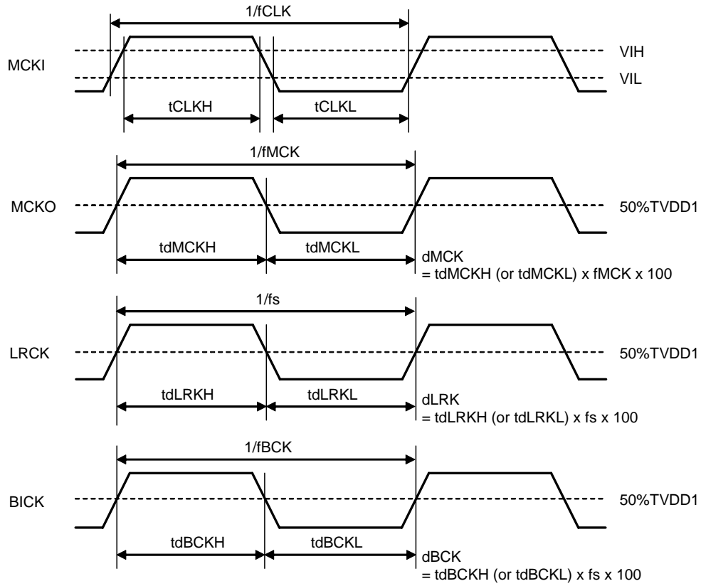
Figure 5. Clock Timing (TDM1/0 bit = "00" & Master mode)
