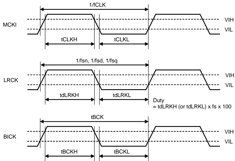
Figure 3. Clock Timing (TDM1/0 bit = "00" &amp; Slave mode)
