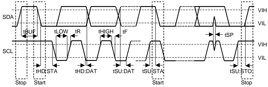
Figure 15. I 2 C Bus mode Timing
