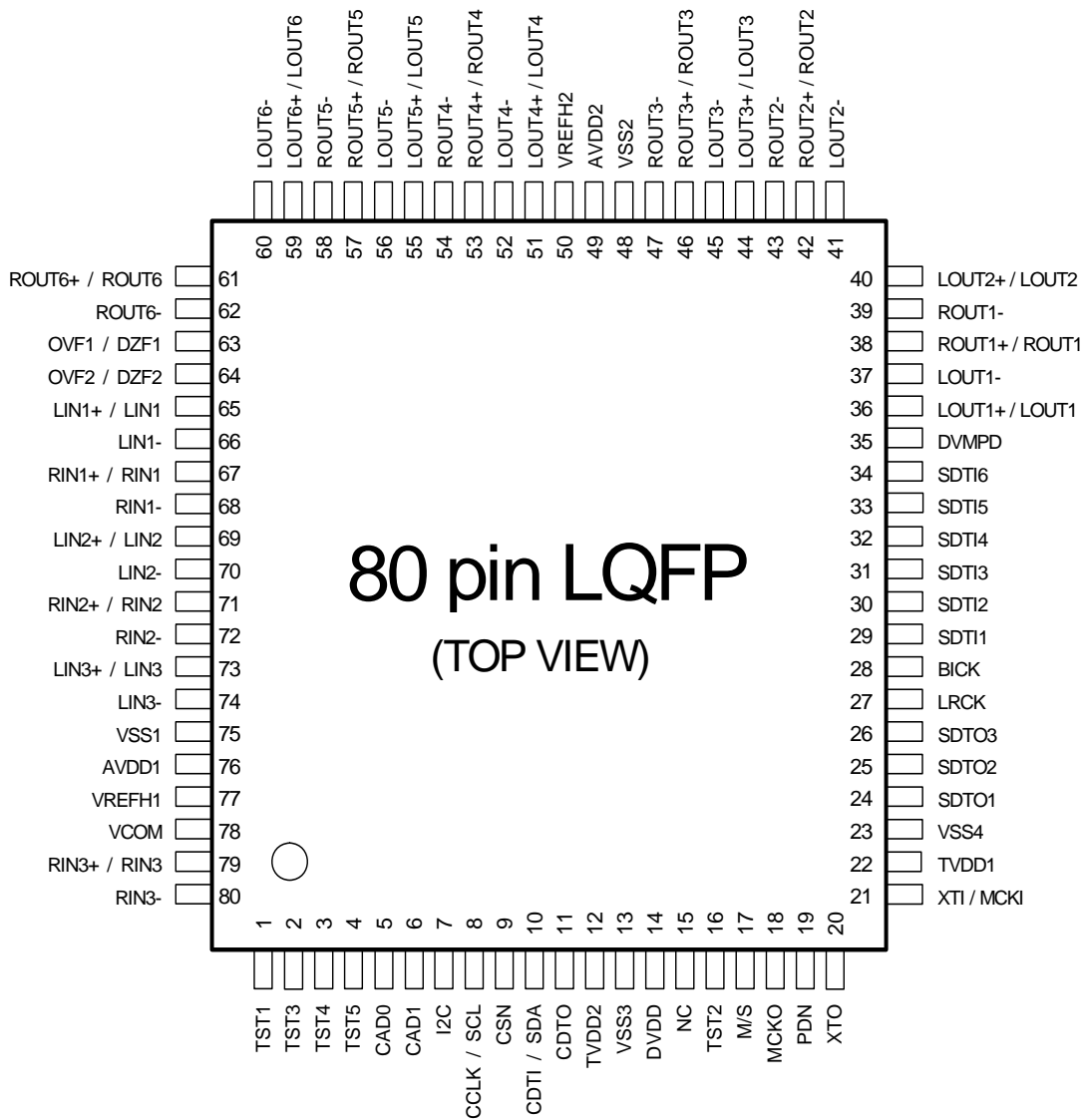
Figure 2. Pin Layout
