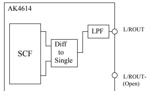
Figure 22. Single-end Output (DOE1-6 bit = “0”)
