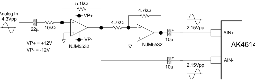
Figure 62. Input buffer circuit example 2 (AC coupled single-end input)
