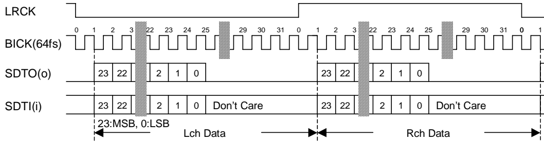
Figure 27. Mode 4/9 Timing (Stereo Mode)
