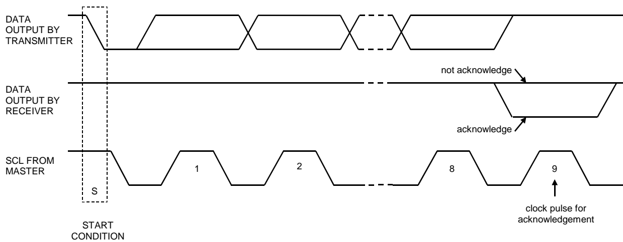
Figure 57. Acknowledge on the I 2 C-Bus
