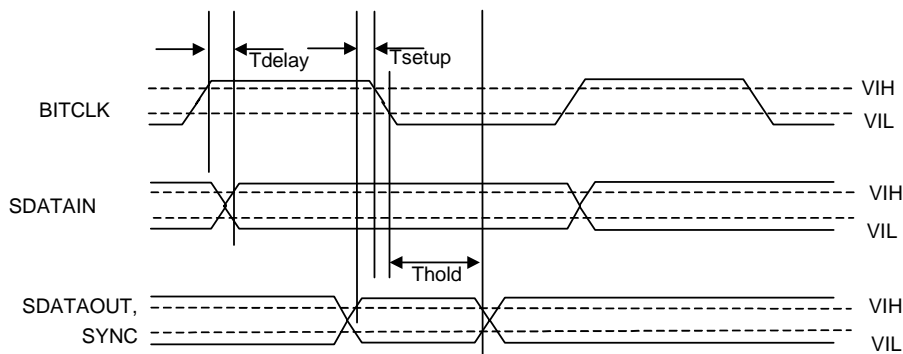
Figure 5. Setup and Hold Timing
