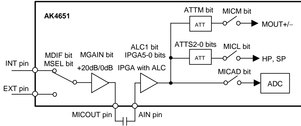
Figure 15. Microphone Input
