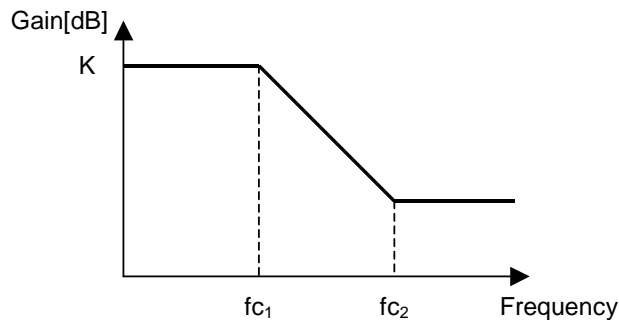
Figure 28. EQ0 Frequency Response
