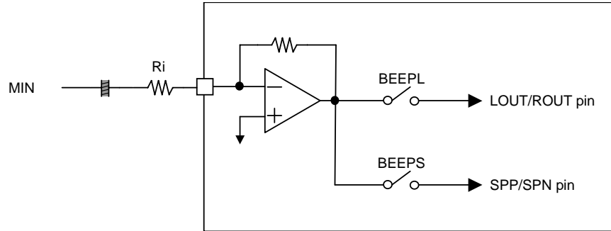
Figure 7. Block Diagram of MIN pin
