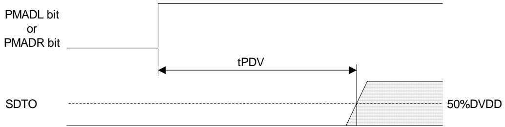
Figure 9. Read Data Output Timing
