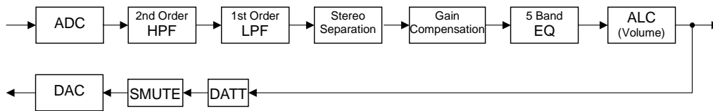
Figure 27. Path at Loop Through Mode
