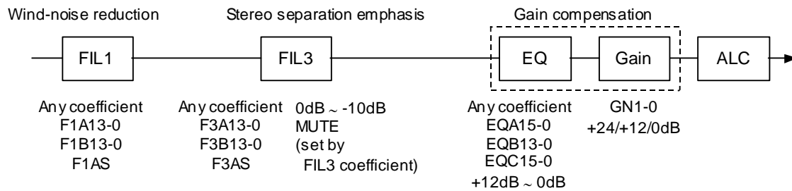
Figure 24. Digital EQ/HPF/LPF
