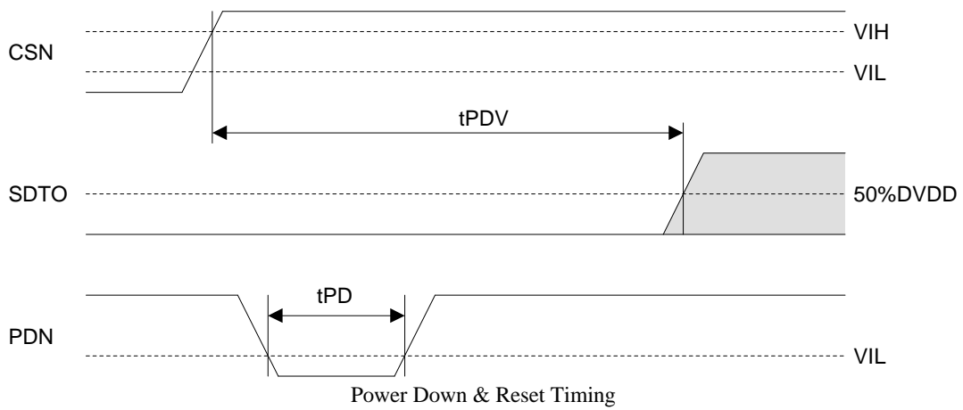
I 2 C Bus Mode Timing
