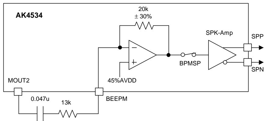
Figure 16. Connection example for 300mW output using BEEPM pin
