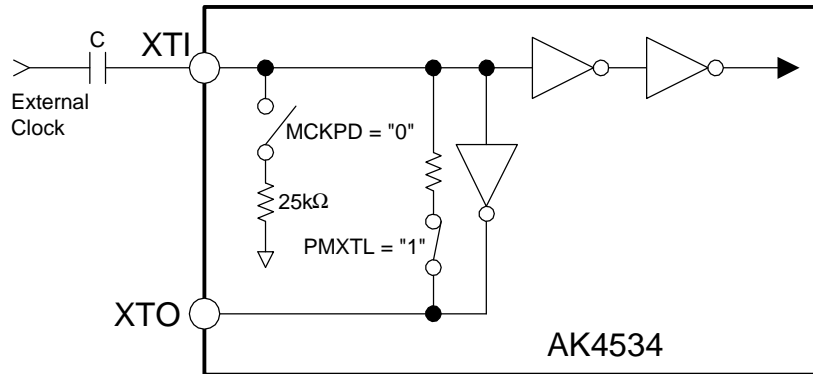
Figure 5. External Clock mode (Input : \geq 50\%DVDD ) - Note: This clock level must not exceed DVDD level. (C : 0.1μF)
