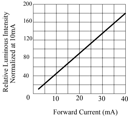
Fig.1 RELATIVE LUMINOUS INTENSITY VS. FORWARD CURRENT
