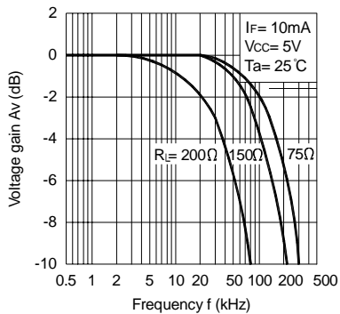
Fig.11 Frequency Response
