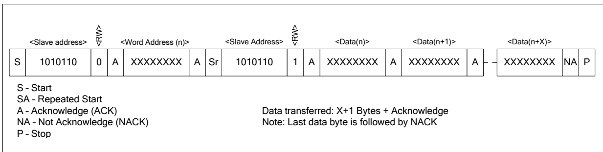
Figure 9. Data Read (Write Pointer, Then Read) - Slave Receive and Transmit
