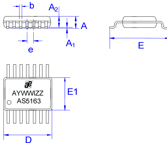
Figure 30: Package Dimensions and Marking
