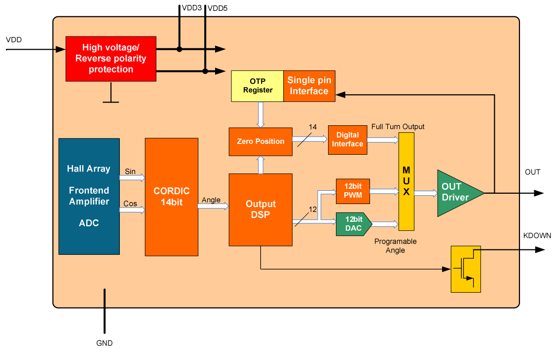
Figure 2: Block diagram AS5163
