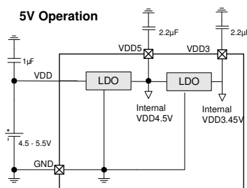
Figure 4: Connections for 5V supply voltages
