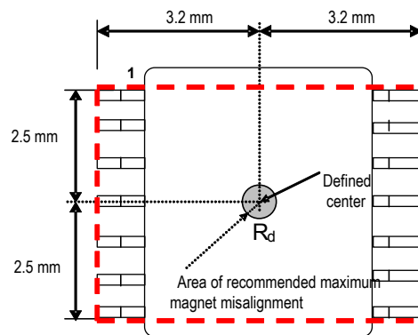
Figure 28: Defined chip center and magnet displacement radius
