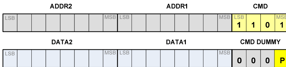
Figure 25: Frame organisation of the READ command
