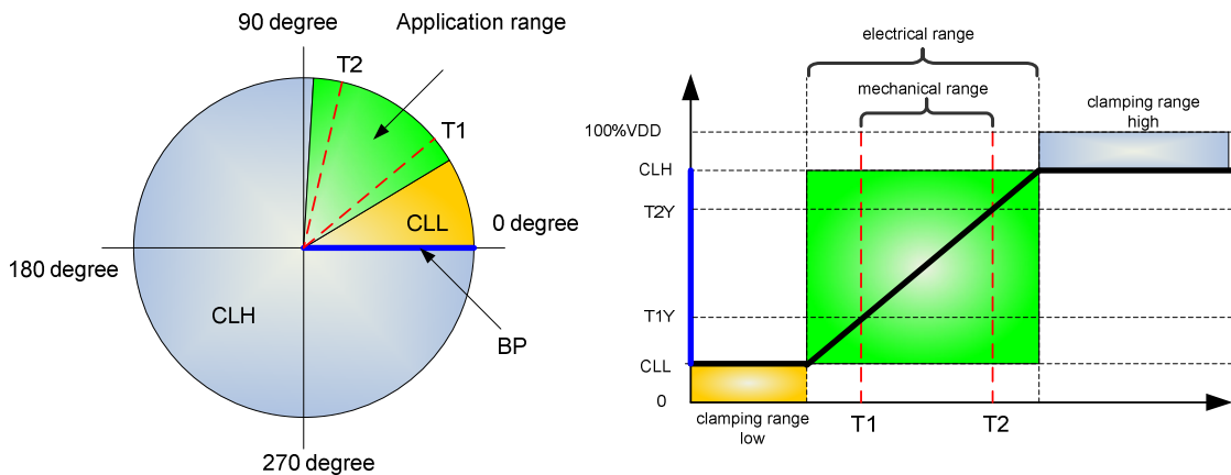
Figure 5: Programming of an individual application range
