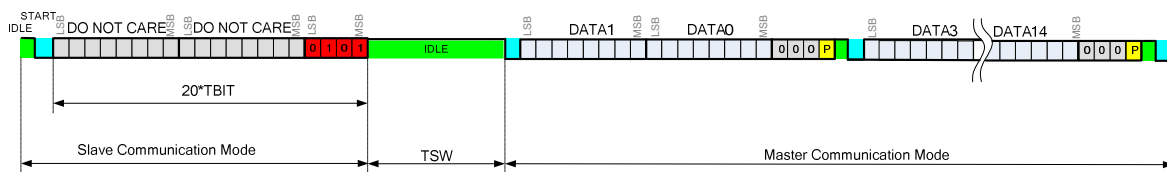
Figure 16: Bus timing for the READ128 command
