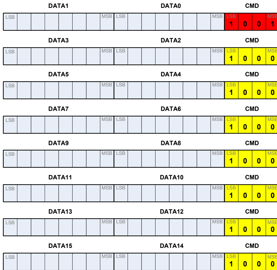
Figure 19: Frame organisation of the WRITE128 command
