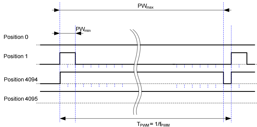
Figure 9: PWM output signal
