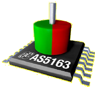
Figure 1: Typical arrangement of AS5163 and magnet
