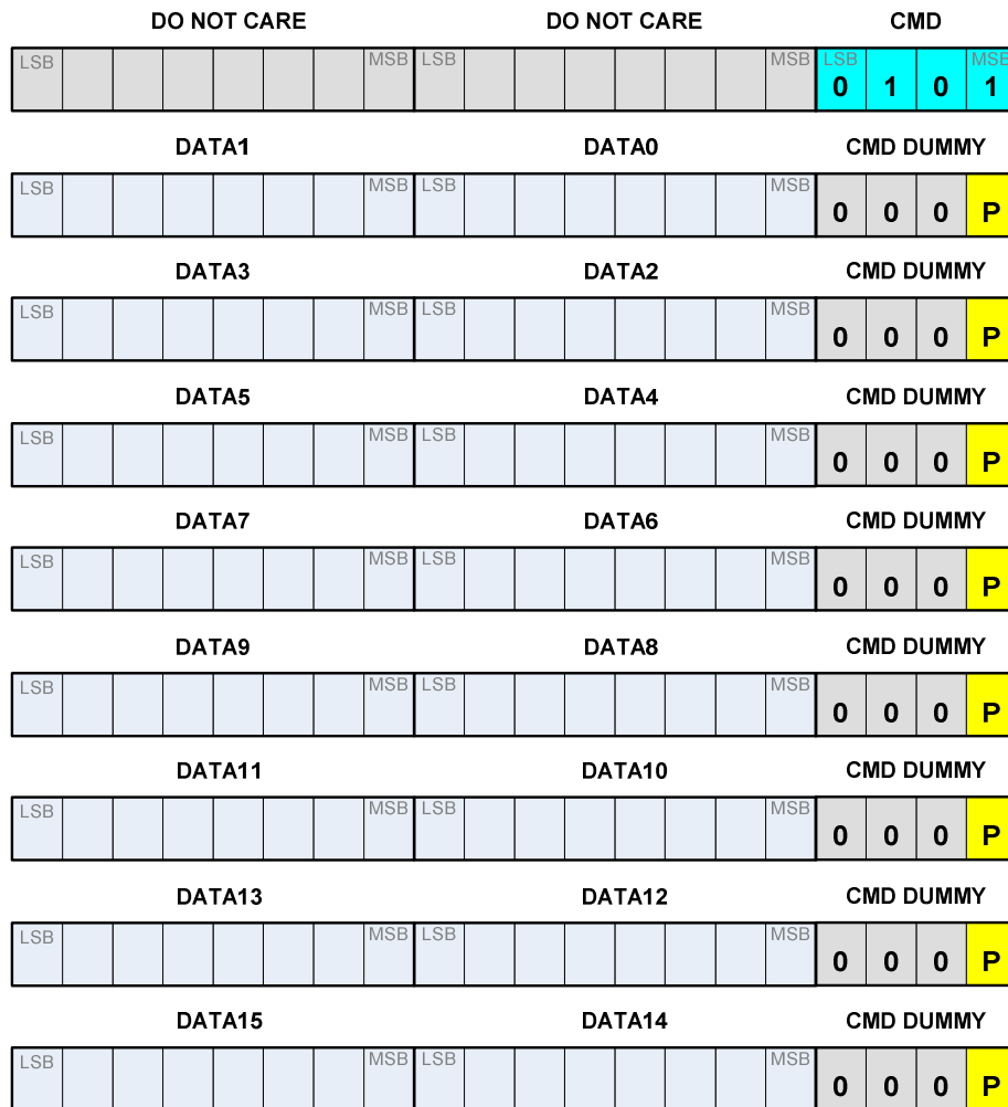
Figure 20: Frame organisation of the READ128 command
