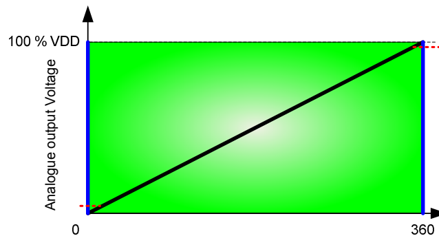
Figure 7: Full scale mode
