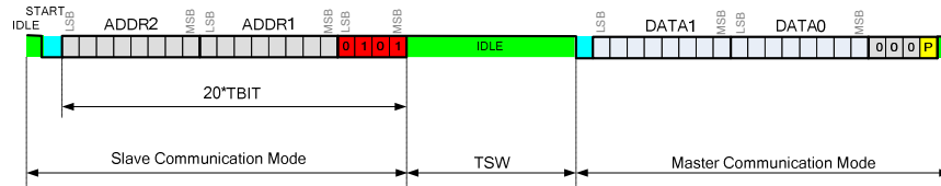
Figure 17: Bus timing for the READ commands
