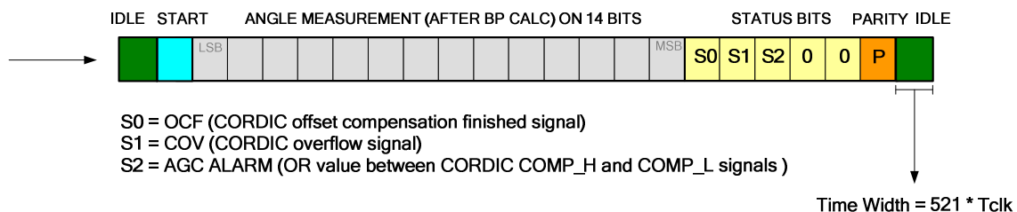
Figure 10: Frame of digital protocol mode
