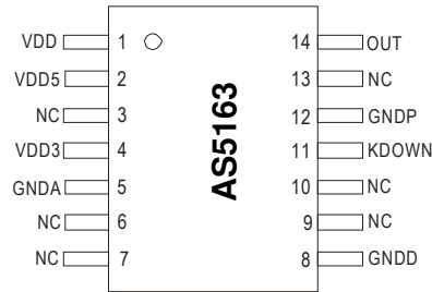
Figure 3: Pin configuration TSSOP14
