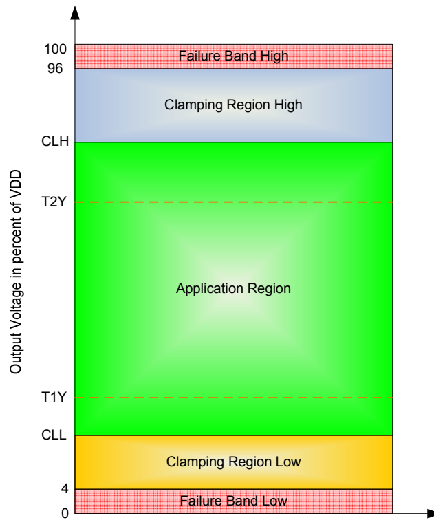
Figure 8: Overview about the angular output voltage
