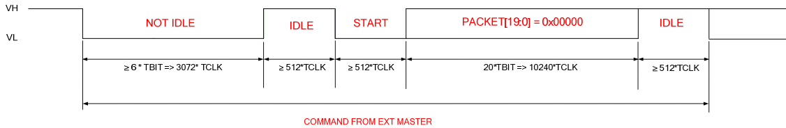
Figure 18: Unblock sequence
