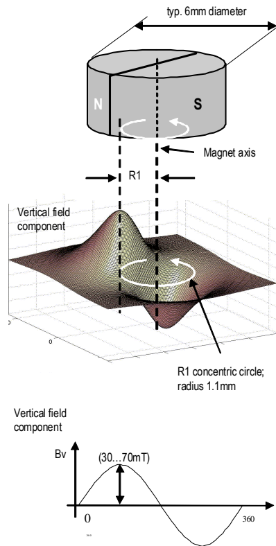
Figure 27: Typical magnet (6x3mm) and magnetic field distribution
