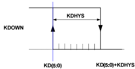
Figure 11: Kick Down Hysteresis implementation
