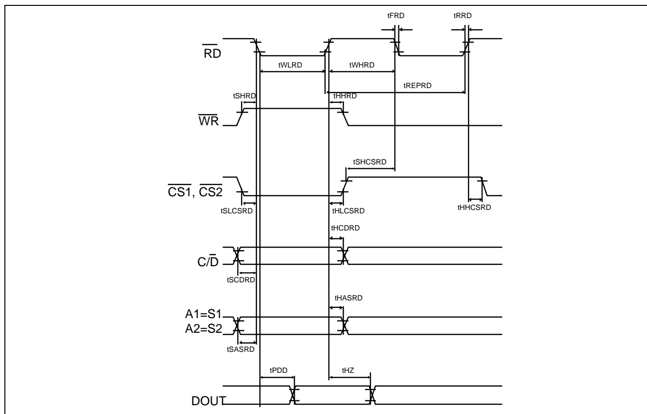
Figure 7 Read Timing
