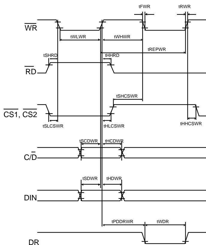
Figure 6 Write Timing
