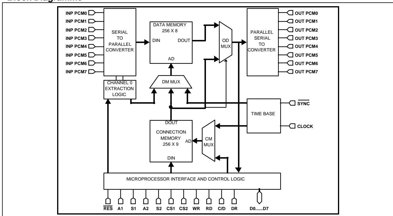
Figure 1: Block Diagramme
