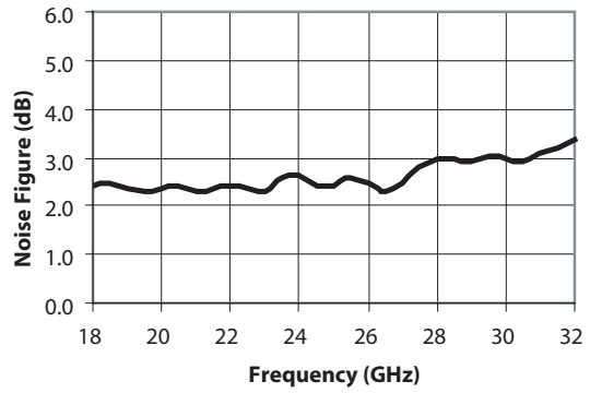
Figure 2. Noise Figure
