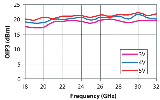
Figure 12. Output IP3 over Vdd
