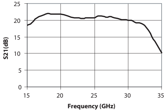
Figure 1. Gain
