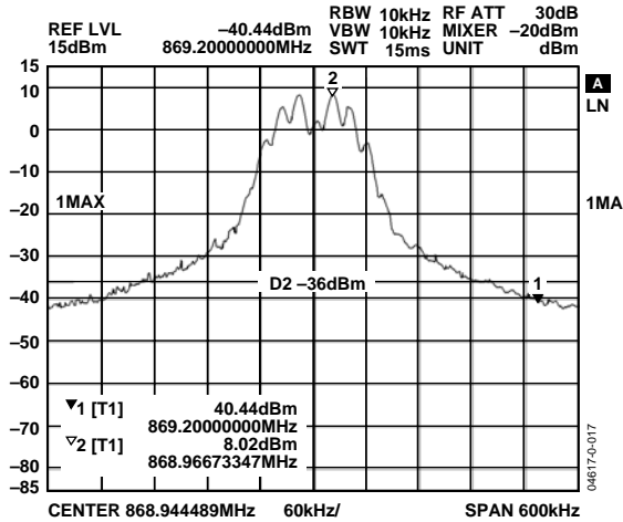
Figure 17. FSK Modulation, Power = 12.5 dBm, Data Rate = 38.4 kbps, F_{\text{DEVIATION}} = \pm 19.2 \text{ kHz}
