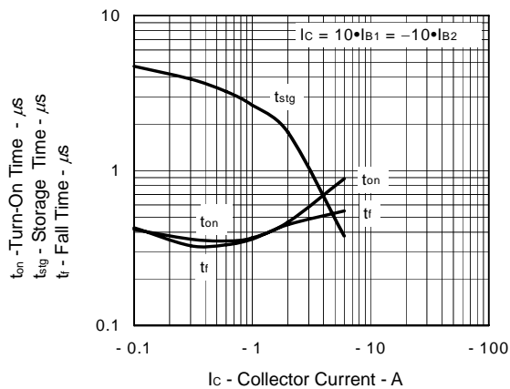
SWITCHING CHARACTERISTICS
