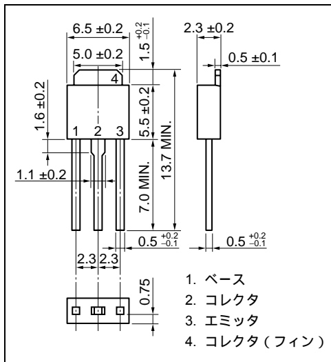
1) TO-251 (MP-3)
