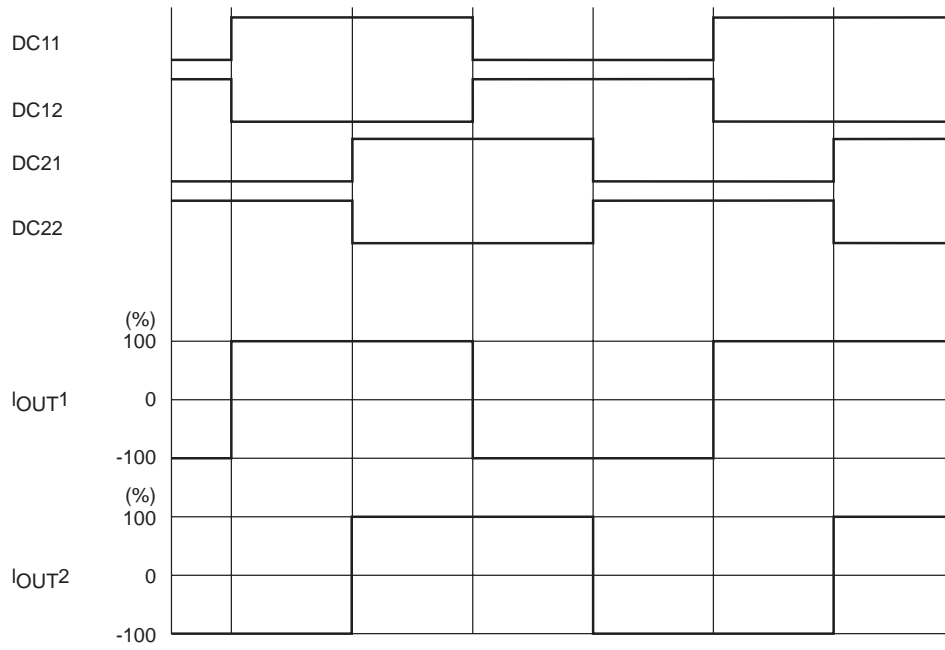
(5) Typical current waveform in each excitation mode when stepping motor parallel input control 2-phase excitation (CW mode)
