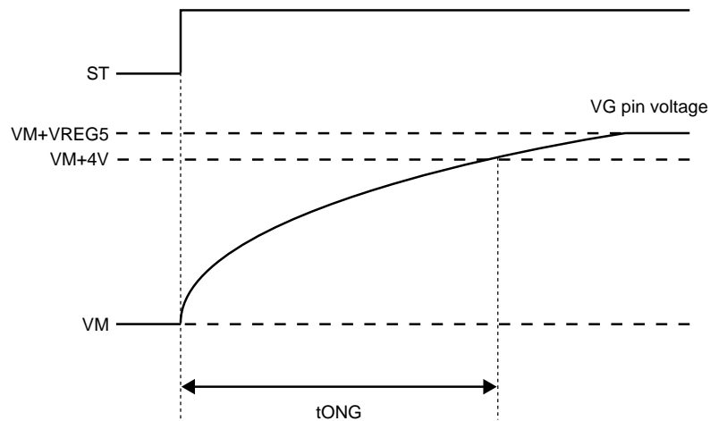
VG Pin Voltage Schematic View
