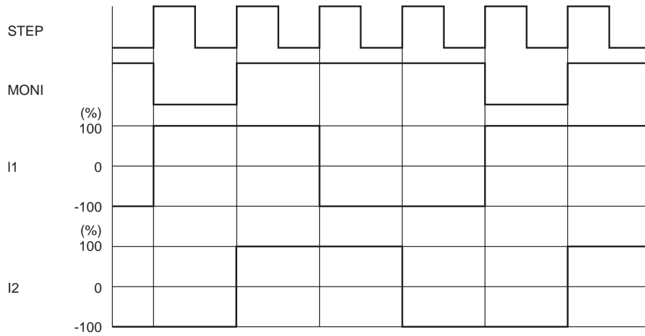
(10) Typical current waveform in each excitation mode 2-phase excitation (CW mode)
