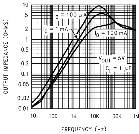
Output Impedance
