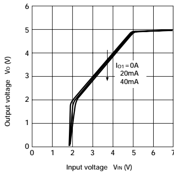
■ Rise Characteristics
