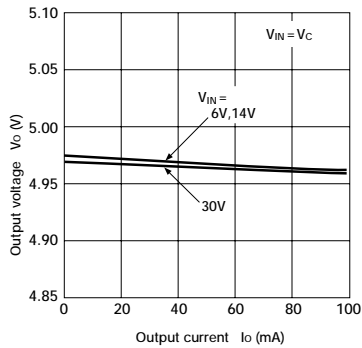
■ Load Regulation (2)
