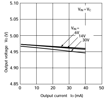
■ Load Regulation (1)
