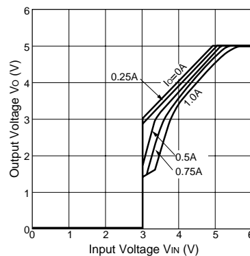
Rise Characteristics(SI-3050N)
