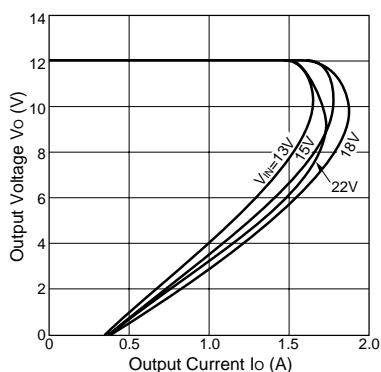
Overcurrent Protection Characteristics(SI-3120N)
