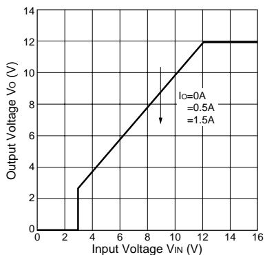
Rise Characteristics(SI-3120N)
