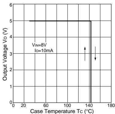
Thermal Protection Characteristics(SI-3050N)
