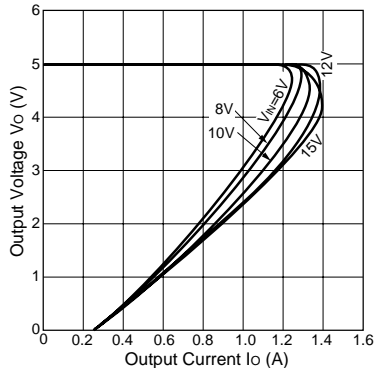
Overcurrent Protection Characteristics(SI-3050N)
