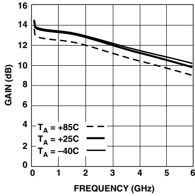
Figure 1. Power Gain vs. Frequency and Temperature.
