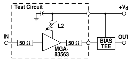
Figure 44. L2 Test Circuit.
