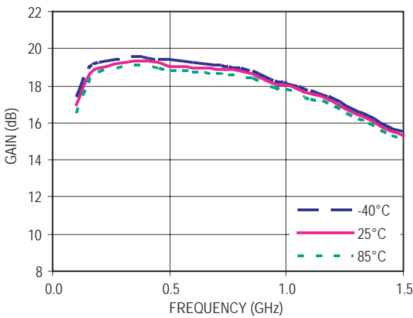
Figure 14. Gain vs Frequency ( V_d = 3V , I_{ds} = 10mA )
