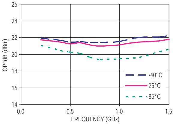
Figure 33. OP1dB vs Frequency ( V_d = 5V , I_{ds} = 10mA )
