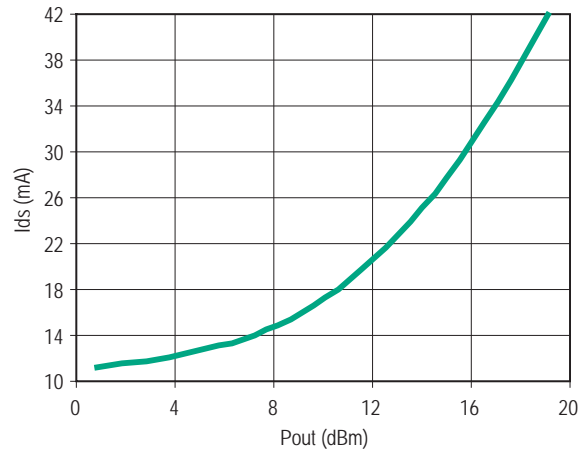
Figure 54. I_{ds} vs Pout ( V_d = 5\text{V} )
