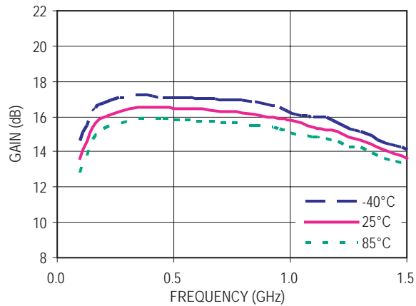
Figure 8. Gain vs Frequency ( V_d = 3V , I_{ds} = 5mA )
