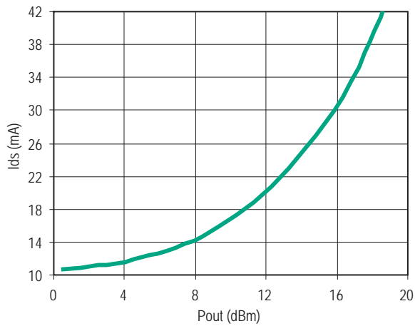
Figure 53. I_{ds} vs Pout ( V_d = 3\text{V} )
