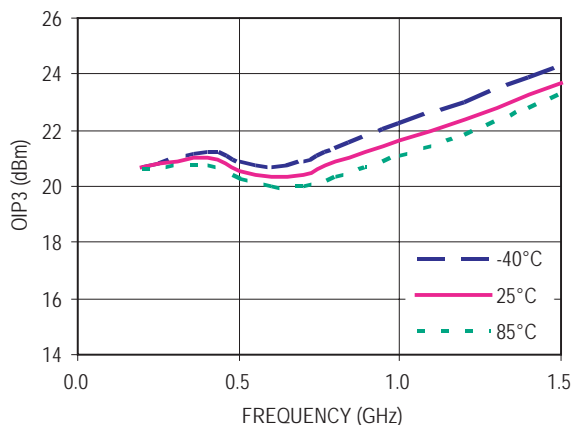
Figure 40. OIP3 vs Frequency ( V_d = 5V , I_{ds} = 15mA )
