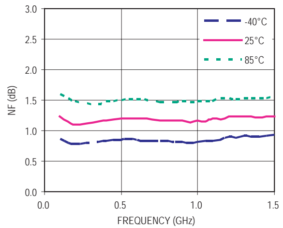
Figure 30. NF vs Frequency ( V_d = 5V , I_{ds} = 5mA )
