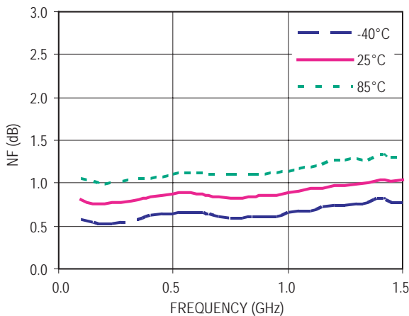
Figure 42. NF vs Frequency ( V_d = 5V , I_{ds} = 15mA )
