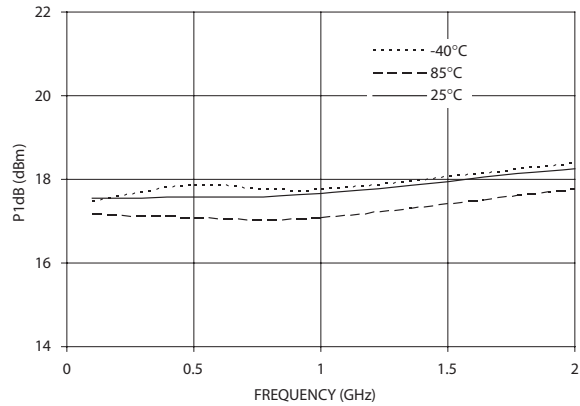
Figure 14. P1dB vs. Frequency (3V,15mA), Ids=15mA during small signal, i.e. Pin=-20dBm)
