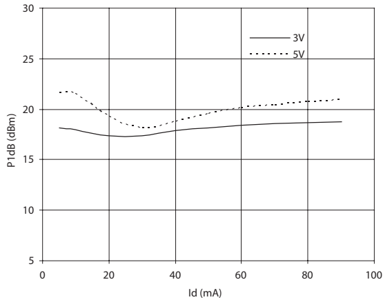
Figure 34. P1dB vs. Id (100MHz), Id at small signal, i.e. Pin=-20dBm
