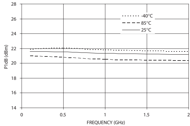
Figure 18. P1dB vs. Frequency (5V,5mA), I_{ds}=5mA during small signal, i.e. P_{in}=-20dBm )
