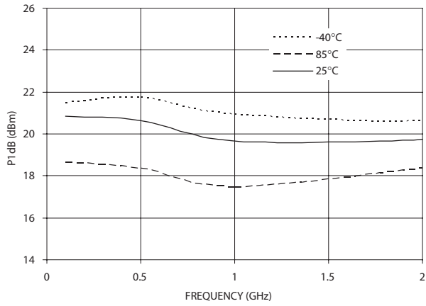
Figure 26. P1dB vs. Frequency (5V,15mA), Ids=15mA during small signal, i.e. Pin=-20dBm)
