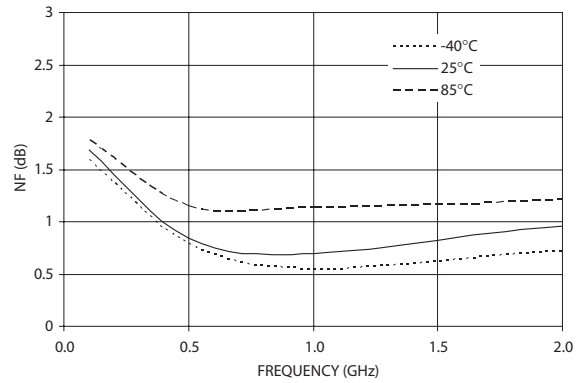
Figure 25. NF vs. Frequency (5V 10mA)
