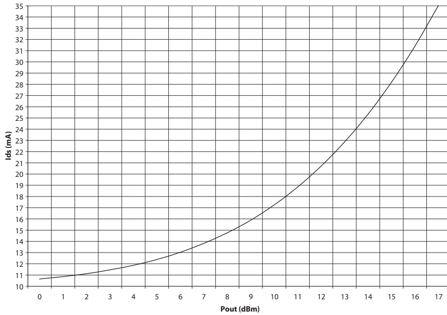
Figure 38. I_{ds} vs. P_{out} ( V_d = 5\text{V} )
