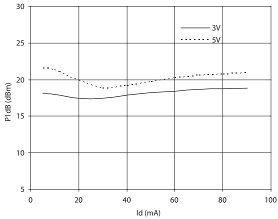
Figure 30. P1dB vs. Id (500MHz), Id at small signal, i.e. Pin=-20dBm)
