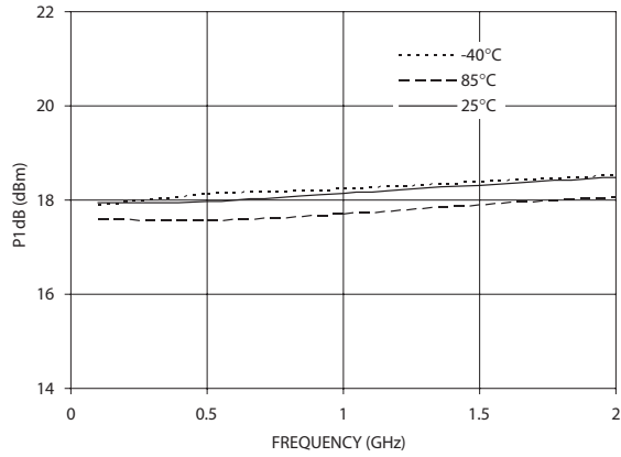
Figure 10. P1dB vs. Frequency (3V,10mA), Ids=10mA during small signal, i.e. Pin=-20dBm)
