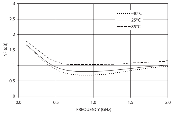
Figure 13. NF vs. Frequency (3V 10mA)
