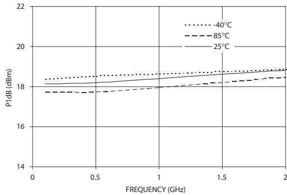
Figure 6. P1dB vs. Frequency (3V,5mA), I_{ds}=5mA during small signal, i.e. P_{in}=-20dBm )
