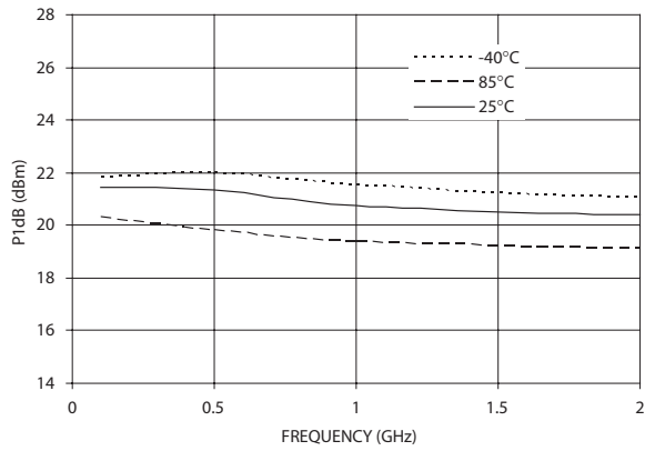
Figure 22. P1dB vs. Frequency (5V,10mA), Ids=10mA during small signal, i.e. Pin=-20dBm)
