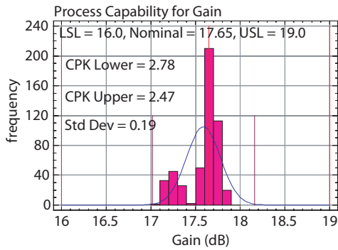
Figure 1. Gain distribution at 60mA
