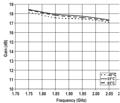
Figure 11. Gain Vs Frequency and Temperature
