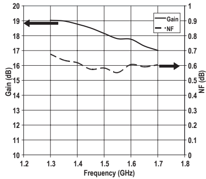
Figure 22. Gain and NF Vs Frequency
