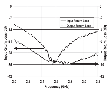
Figure 27. Input and output Return Loss vs Frequency
