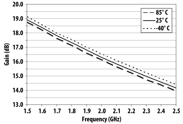
Figure 18. Gain vs Frequency vs Temperature
