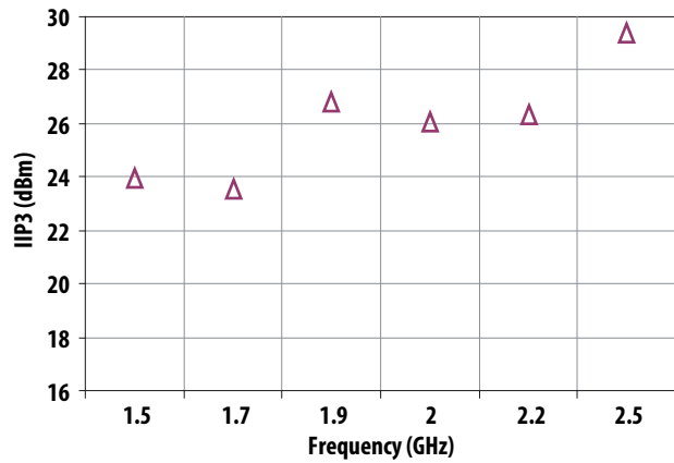
Figure 15. IIP3 vs Frequency for Optimum IIP3 and Fmin at 4.8 V 75 mA
