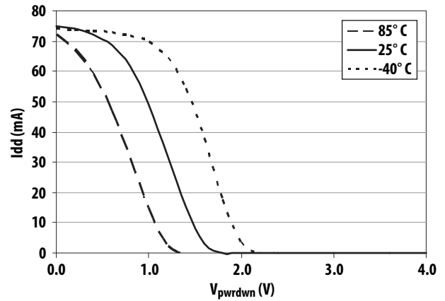
Figure 24. I_{dd} vs V_{pwrdsn}
