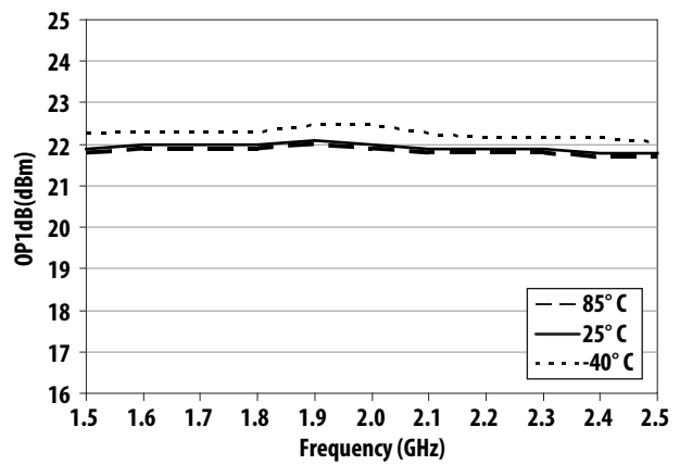
Figure 20. OP1dB vs Frequency vs Temperature
