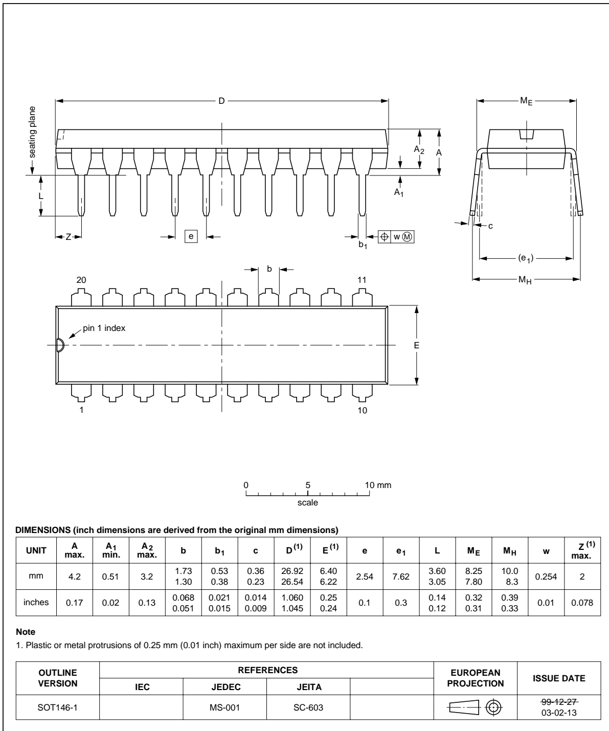
Fig 25. DIP20 package outline (SOT146-1)
