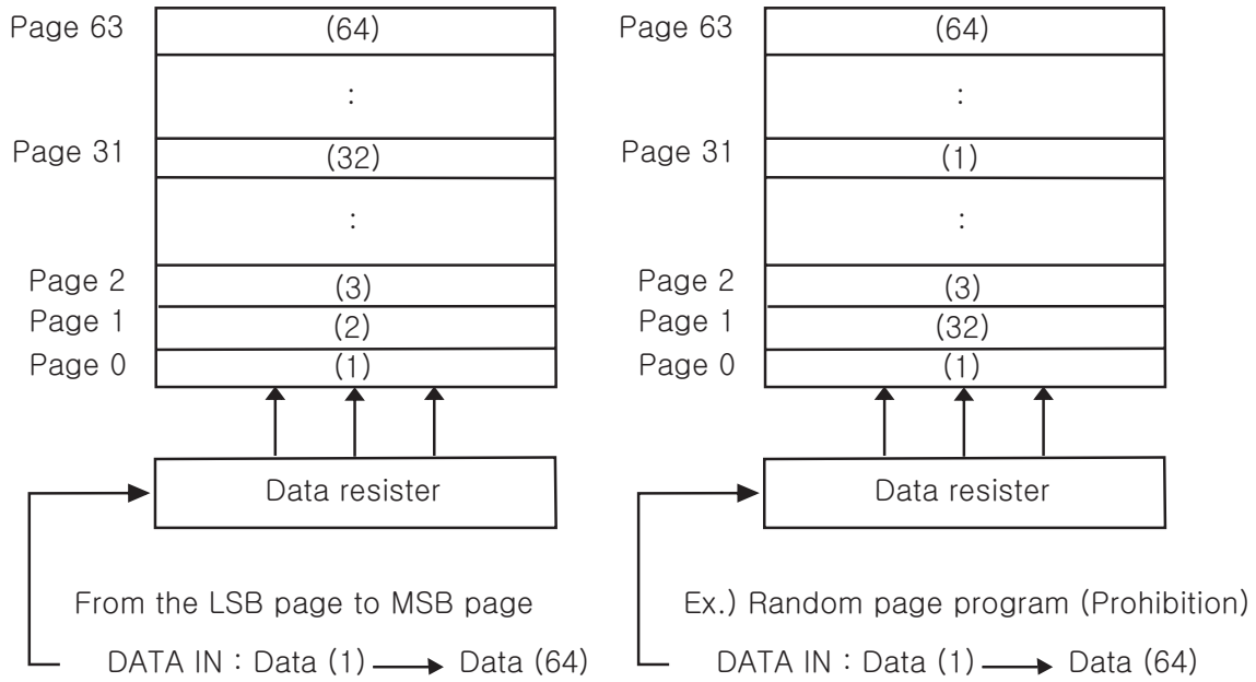
Figure 26: page programming within a block
