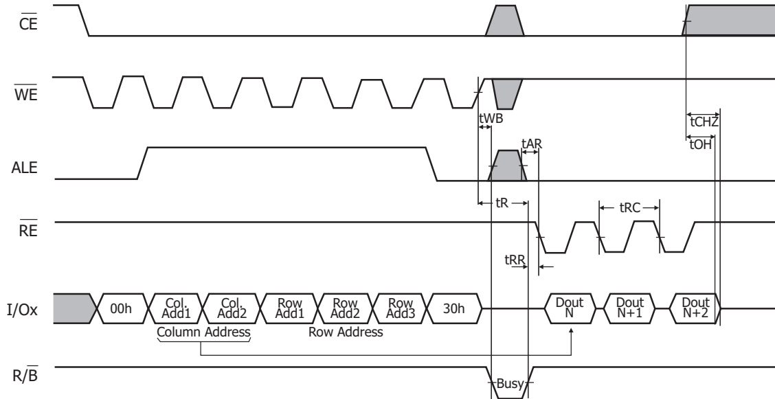
Figure 10: Read1 Operation intercepted by \overline{CE\#}
