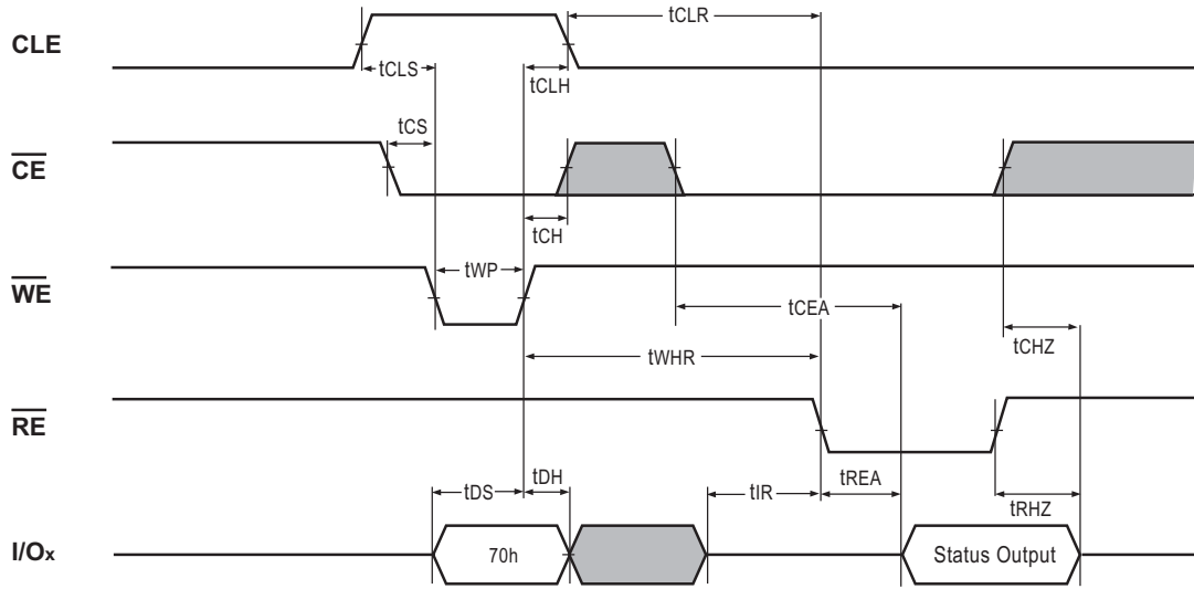
Figure 8: Status Read Cycle
