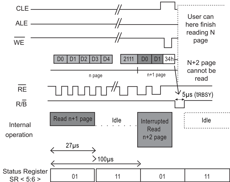
Figure 19: exit from cache read in 5µs when device internally is reading
