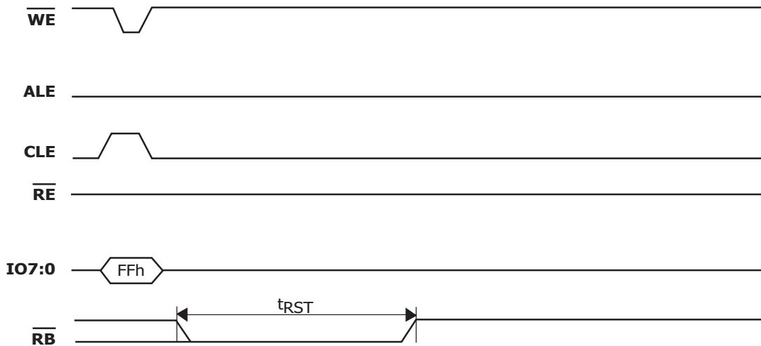
Figure 23: Reset Operation
