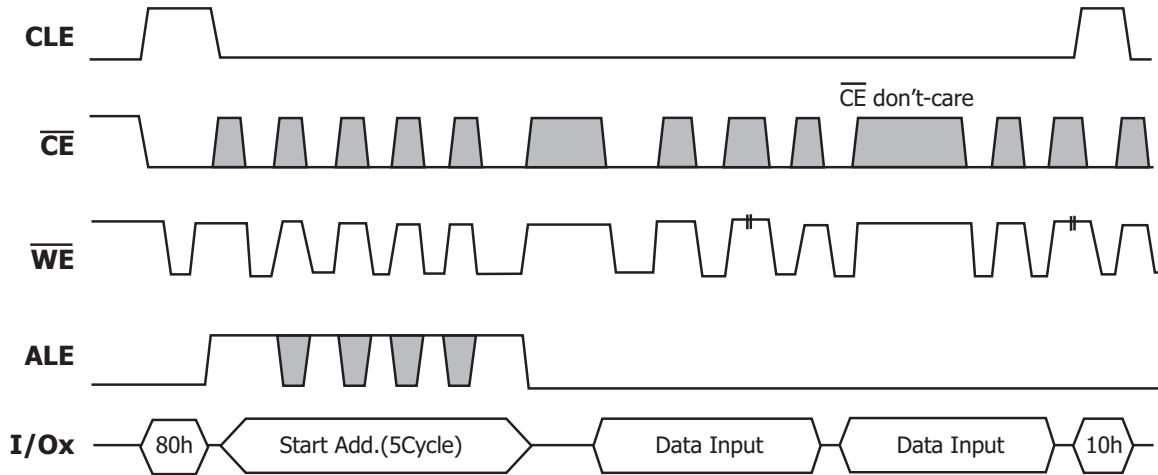
Figure 20: Program Operation with \overline{\text{CE}} don't-care.
