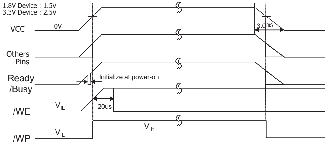
Figure 33: Power-on/off sequence
