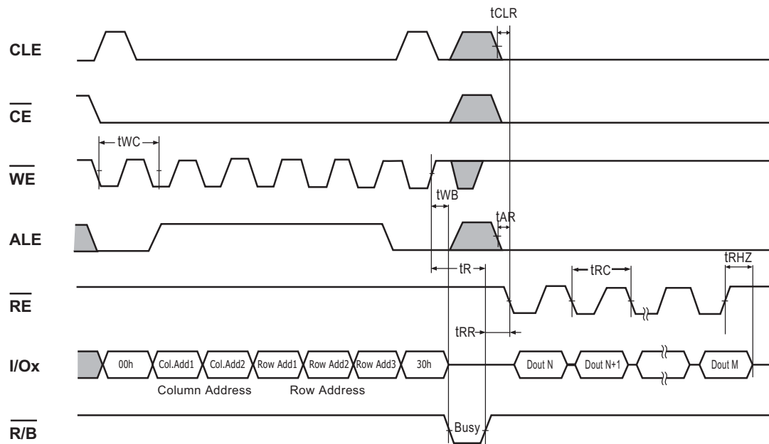
Figure 9: Read1 Operation (Read One Page)
