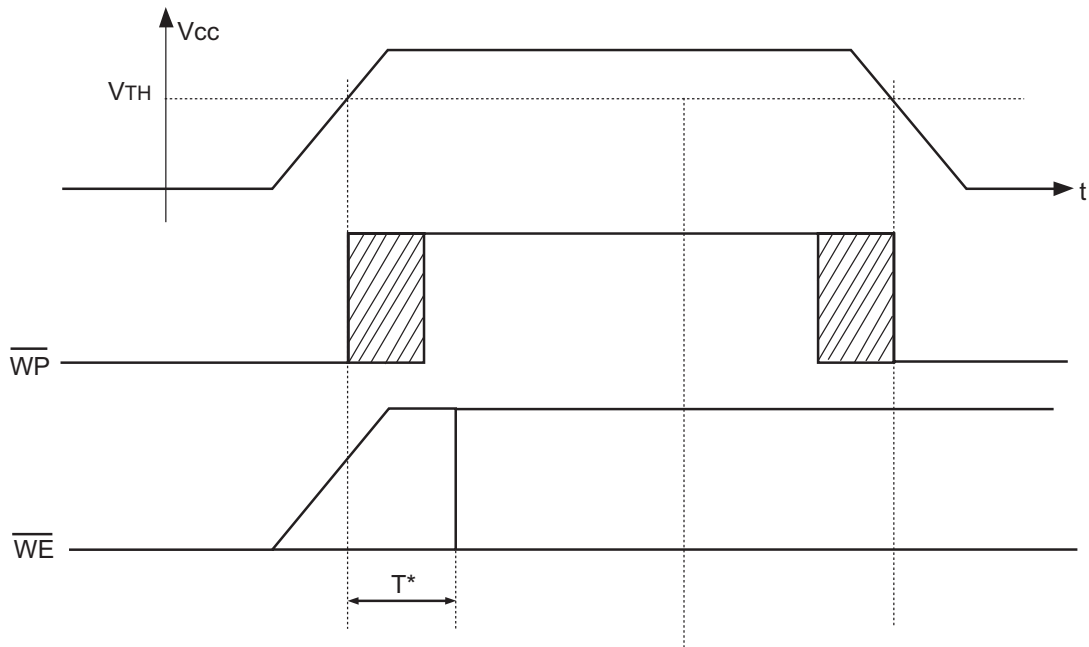
Figure 24: Power On/Off Timing
