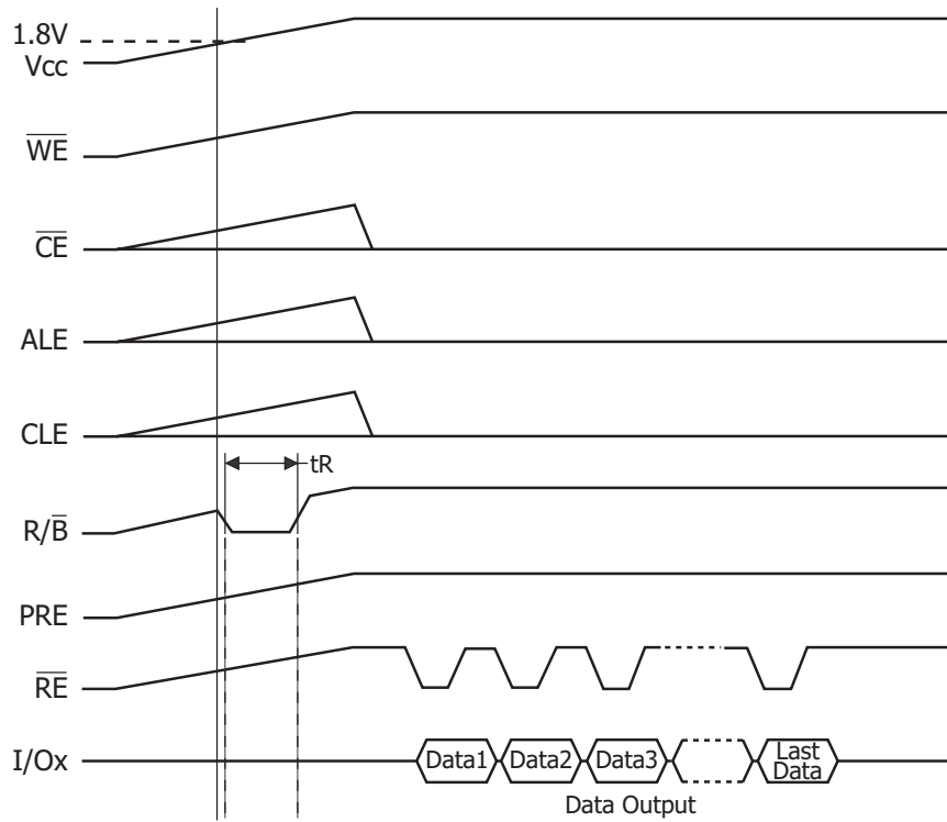
Figure 22: Automatic Read at Power On
