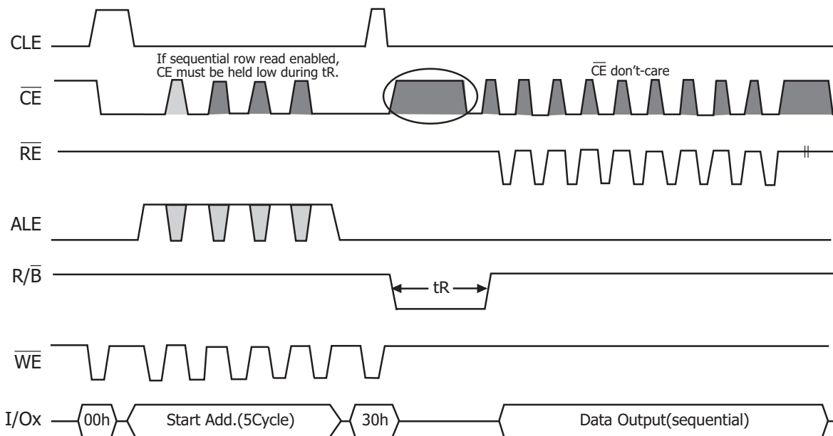
Figure 21: Read Operation with \overline{\text{CE}} don't-care.
