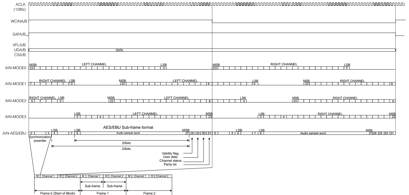
Fig. 1: Audio Input Format Timing Diagram
