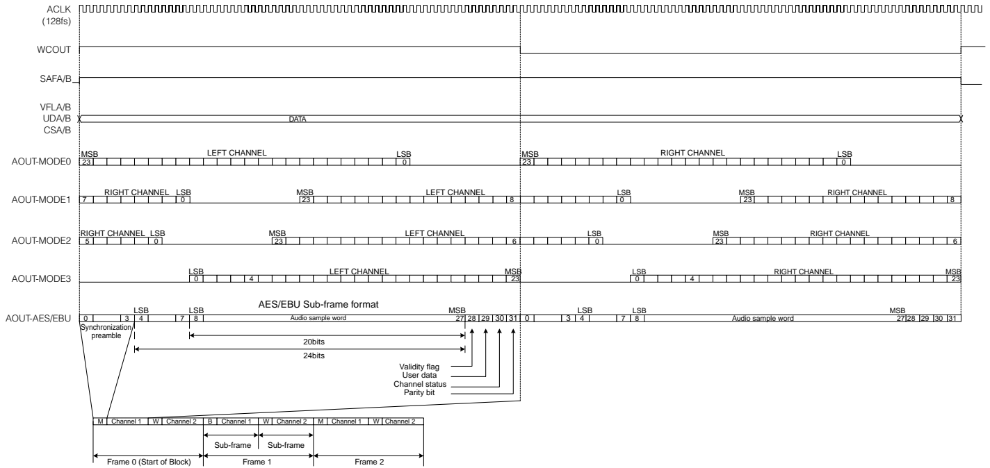
Fig. 12: Audio Data Output Formats
