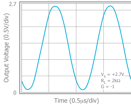
Output Swing
