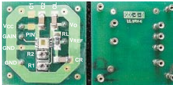
Figure 4. Evaluation Board.
