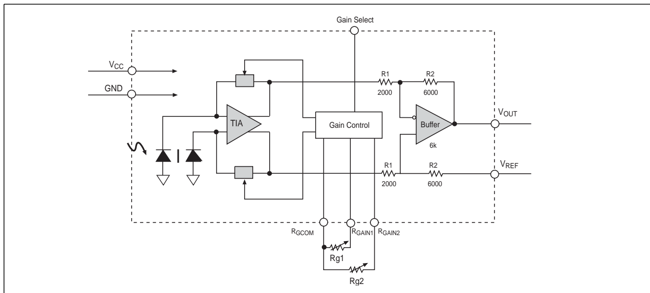
Figure 1. Functional Diagram
