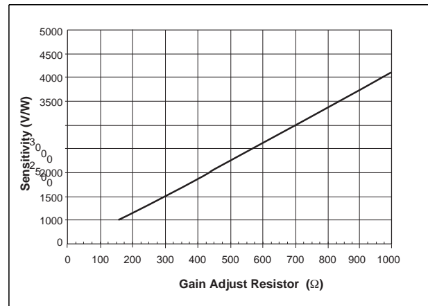
Figure 2. Sensitivity vs. Gain Resistor (Absolute)
