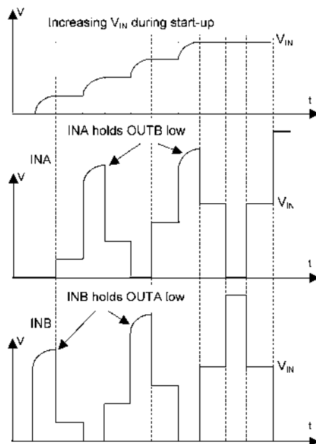
Figure 3. During converter startup, the synchronous MOSFET gate-driver outputs of the SiP11203/SiP11204 are reversed and inverted to prevent spurious MOSFET switching
