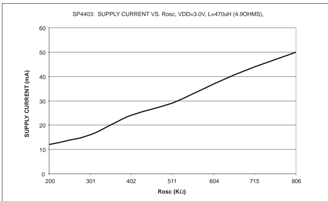
Figure 8. I_{TOTAL} vs R_{osc} , V_{DD}=3.0V , Coil=470\mu H , 4.9\Omega
