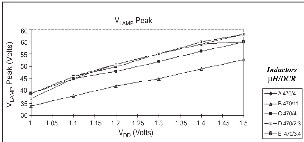
Lamp = 1.5 sq. in., C1 = 0.1μF, C2 = 180pF, D1 = DIN4148
