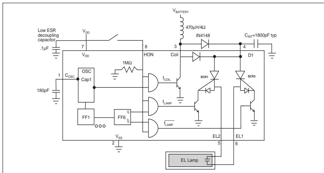
SP4425 Schematic
