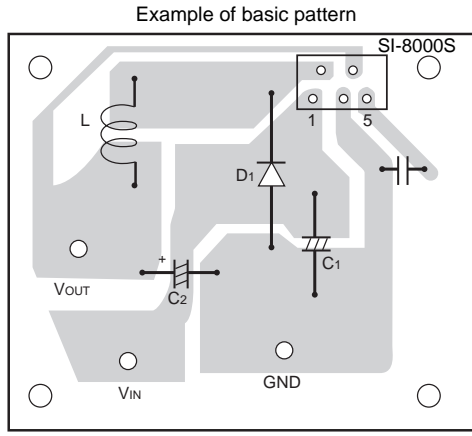
Top view (with part names)
