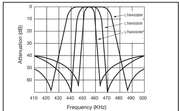
Figure 3) LTM455W – Characteristics
