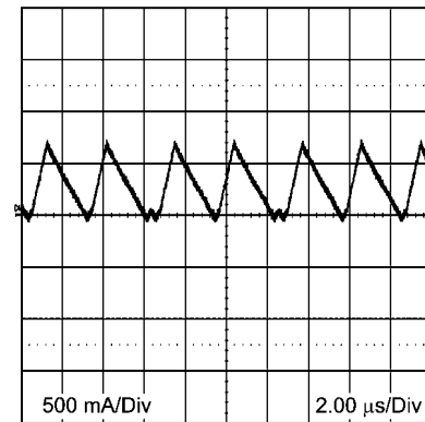
Transition Mode Operation V_{IN} = 24V, V_O = 3.3V, I_O = 0.35A \ 2 \mu\text{sec/div}
