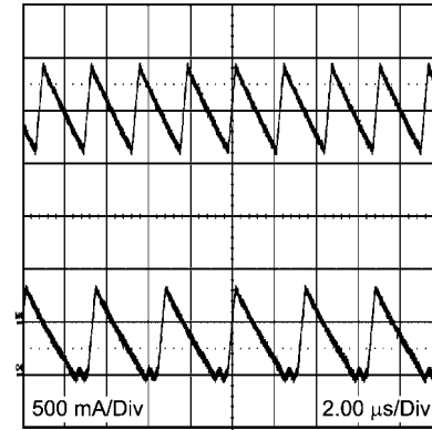
CCM and DCM Operating Modes V_{IN} = 24V, V_O = 3.3V, I_O = 2A/0.32A \ 2 \mu\text{sec/div}
