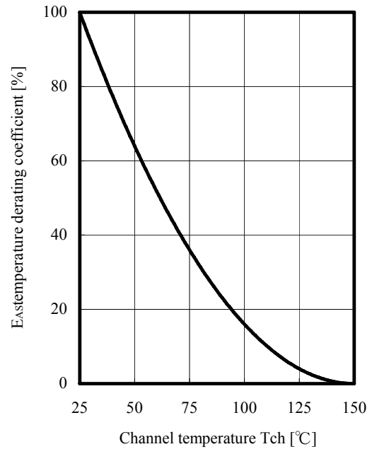
STR-E1555 Fig5 Avalanche energy derating characteristic
