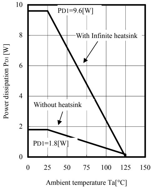
STR-E1555 Fig6 MOSFET Ta-PD1 characteristic
