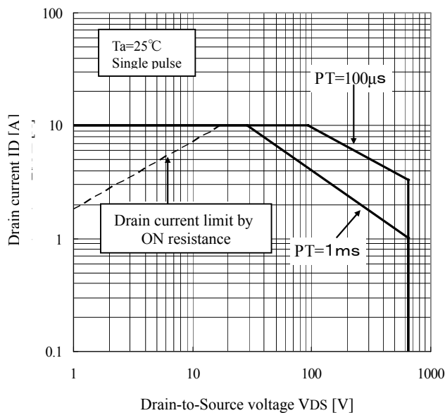
STR-E1555 Fig3 MOSFET A.S.O. characteristic (Ta=25°C/single pulse)
