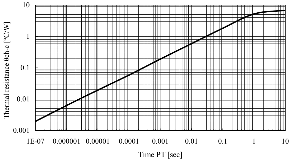
STR-E1555 Fig8 MOSFET Transient thermal resistance characteristic
