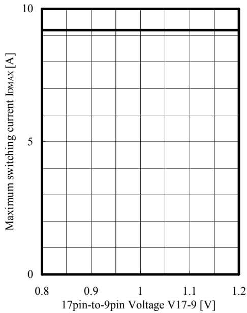
STR-E1555 Fig4 Maximum switching current derating characteristic
