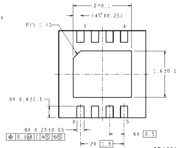
8-Pin LLP NS Package Number SDA08A
