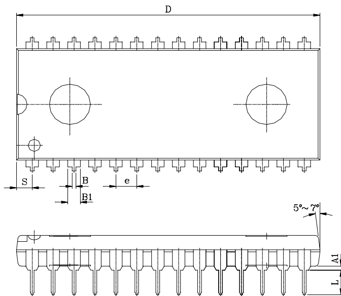
PDIP - 28
