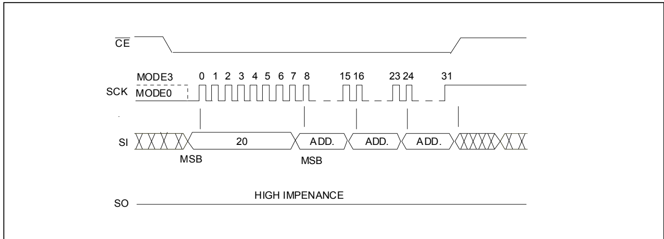
FIGURE 10 : SEQUENCE-ERASE SEQUENCE
