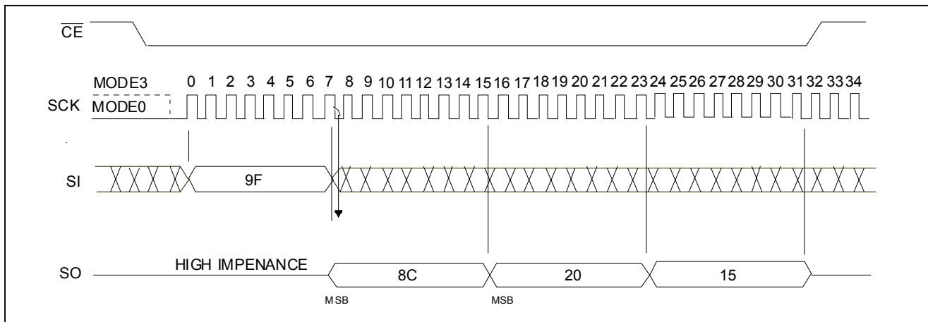
Figure 17 : Jedec-Read-ID Sequence
