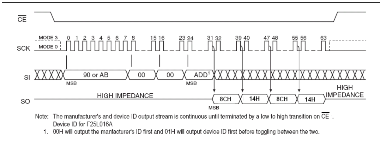
Figure 18 : Read-Electronic-Signature
