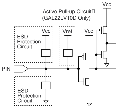
Typical Input
