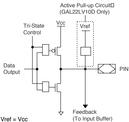
Typical Output
