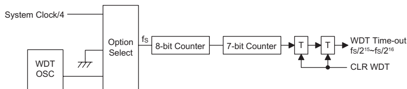
Watchdog Timer
