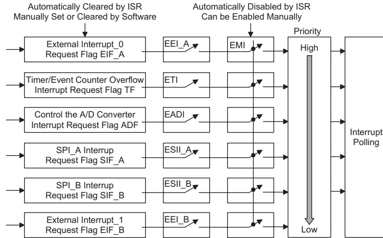
Interrupt Structure
