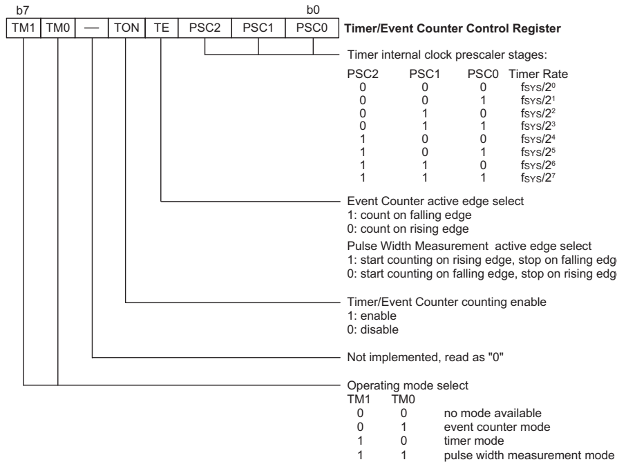
Timer/Event Counter Control Register
