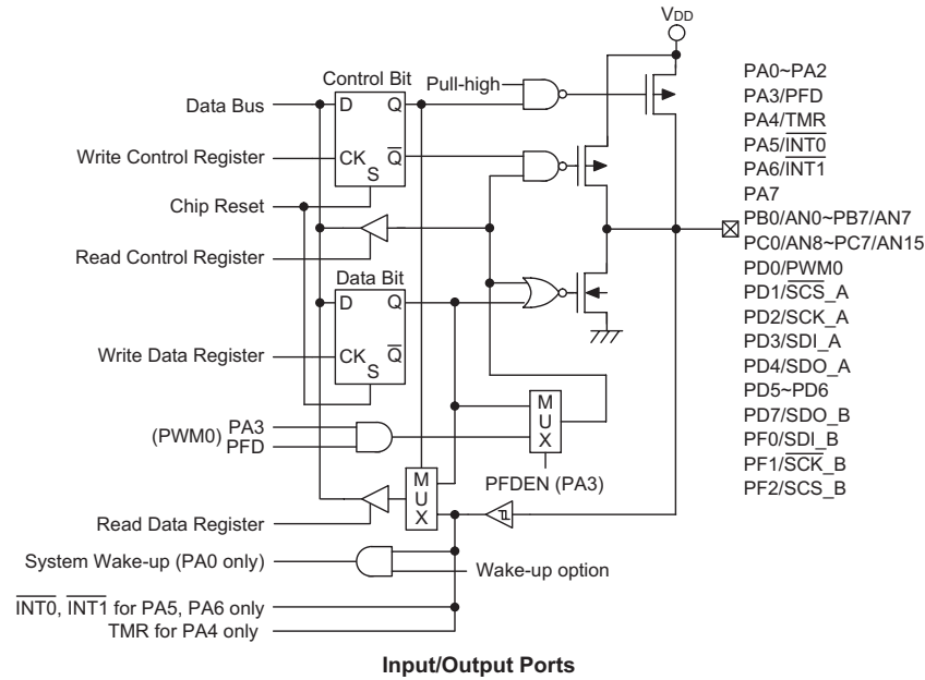
Input/Output Ports
