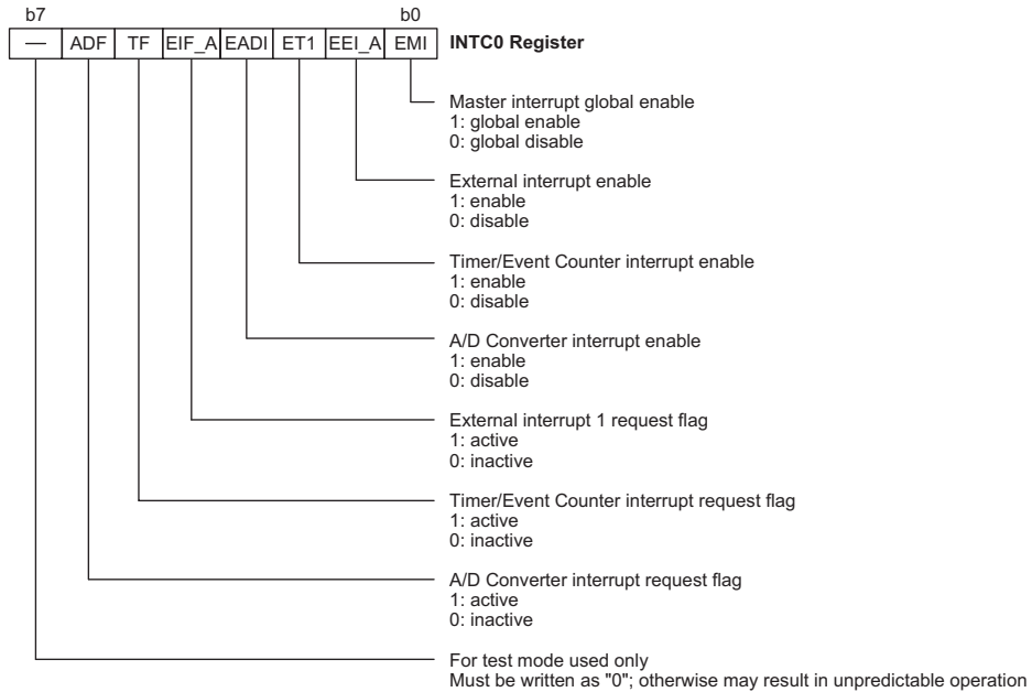
INTC0 Register
