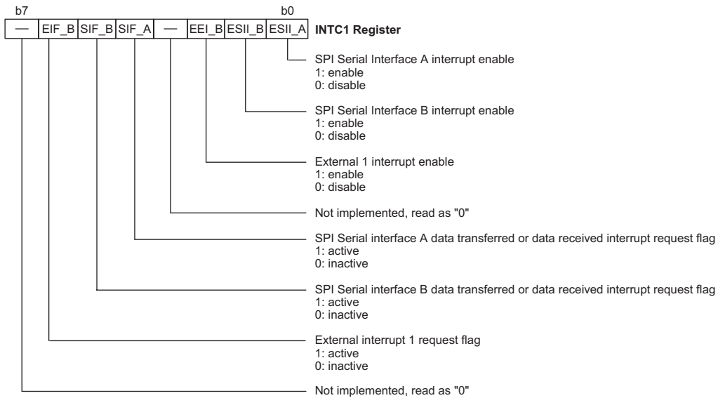
INTC1 Register
