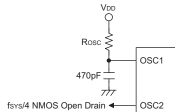
RC Oscillator
