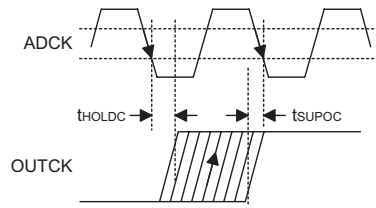
OUTCK Timing Chart
