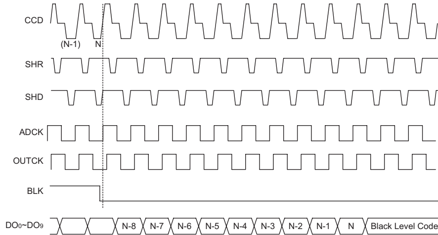
Pixel Data Readout Sequence (2): End of Conversion
