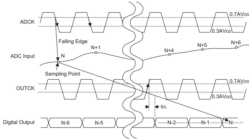
ADC Direct Input Chart
