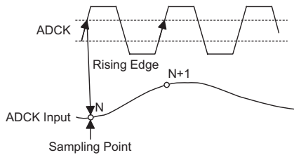
ADCK Inversion Chart
