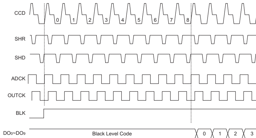
Pixel Data Readout Sequence (1): Start of Conversion
