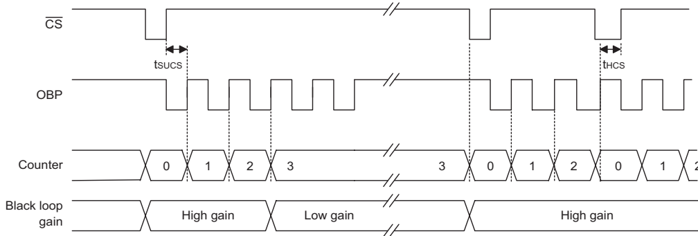
Black Loop Settling Gain Boost Timing
