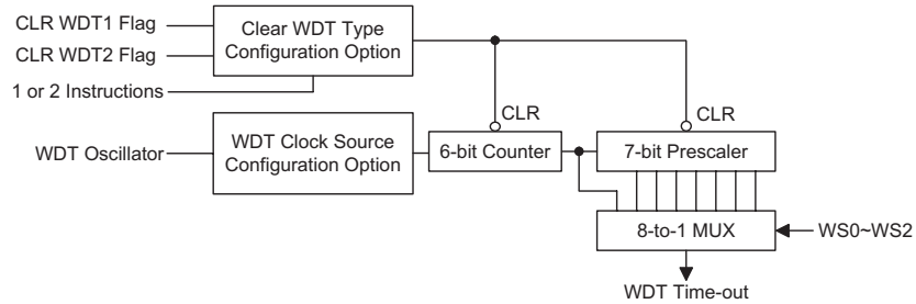
Watchdog Timer
