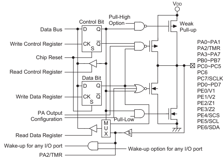
Input/Output Ports
