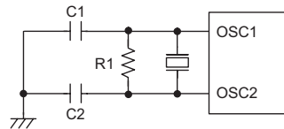
Crystal/Ceramic Oscillator
