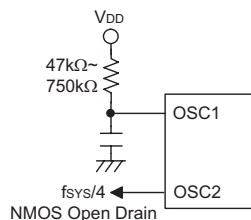
RC Oscillator
