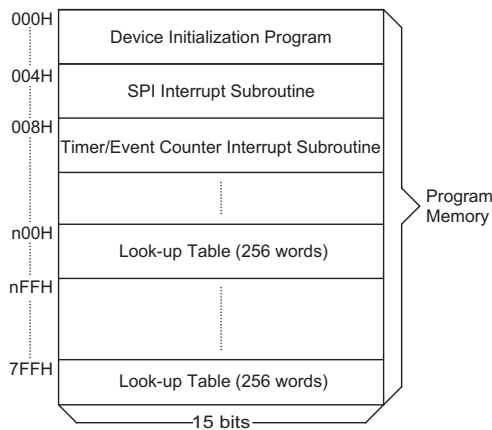
Program Memory Structure
