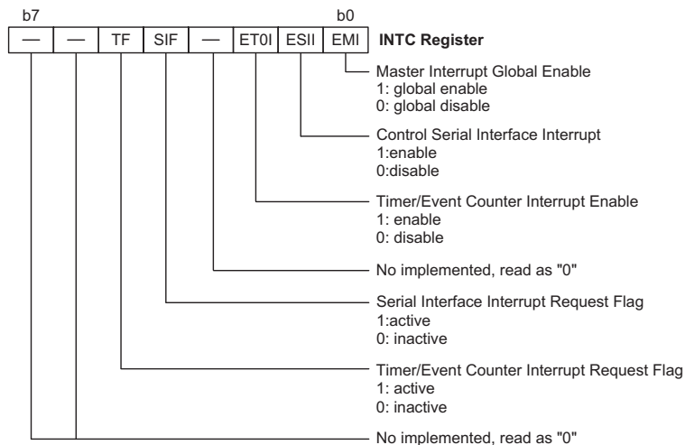
Interrupt Control Register
