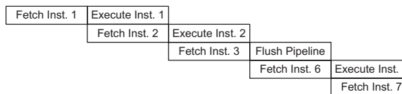
Instruction Fetching
