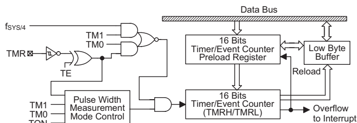
Timer/Event Counter
