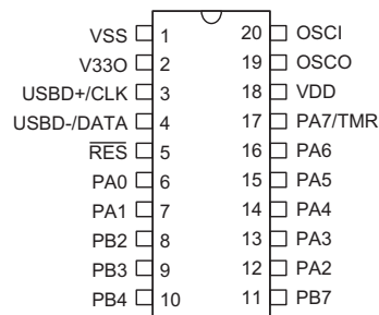
HT82M99E/HT82M99A - 20 DIP-A/SOP-A/SSOP-A
