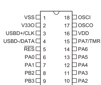
HT82M99E/HT82M99A - 18 DIP-A/SOP-A
